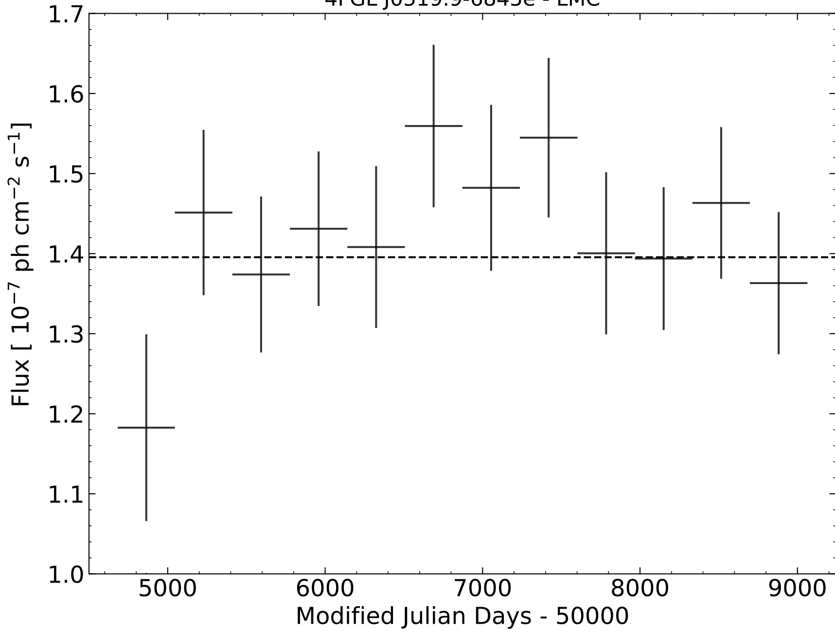
4FGL J0519.9-6845e - LMC
