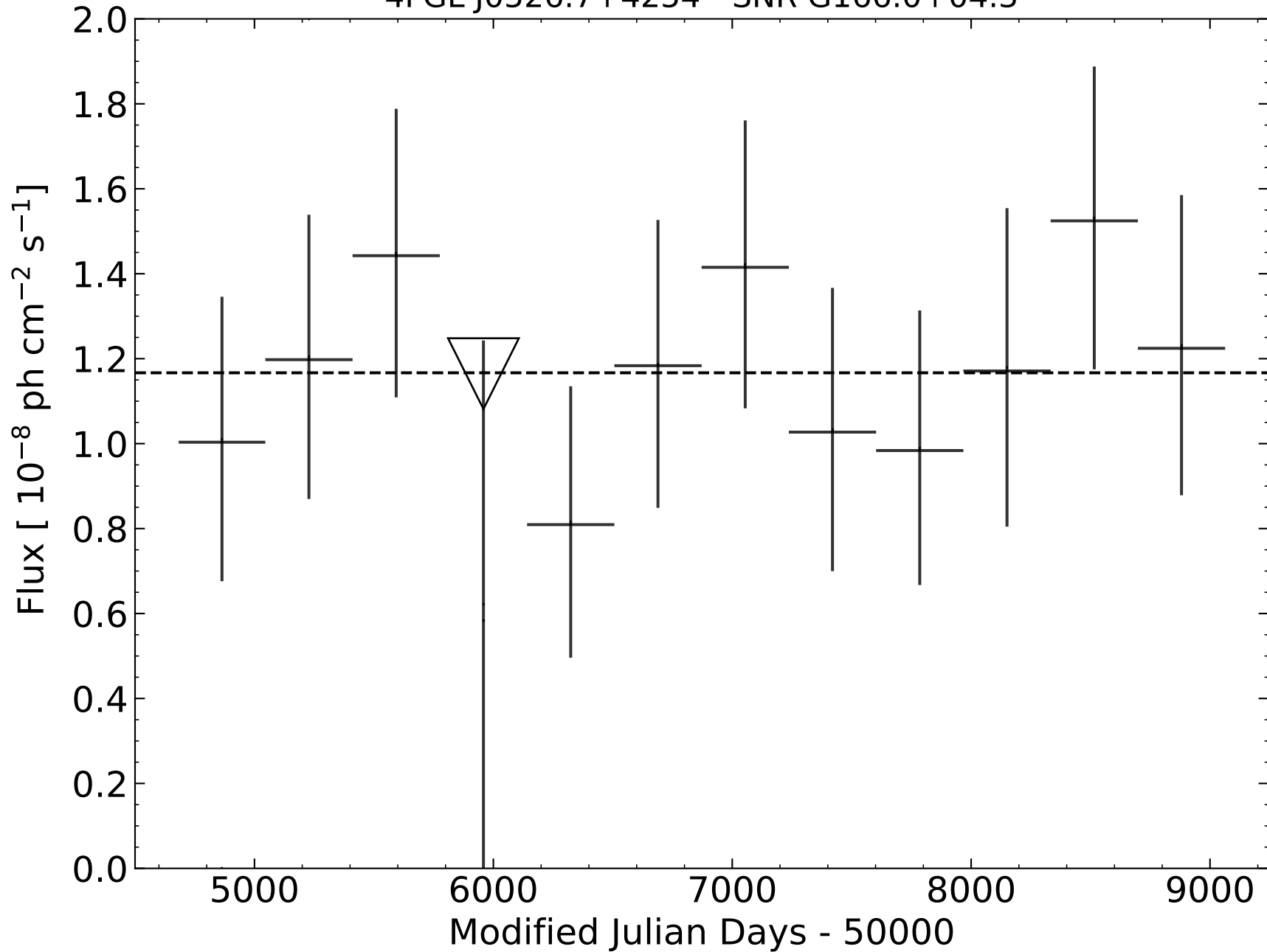
4FGL J0526.7+4254 - SNR G166.0+04.3
