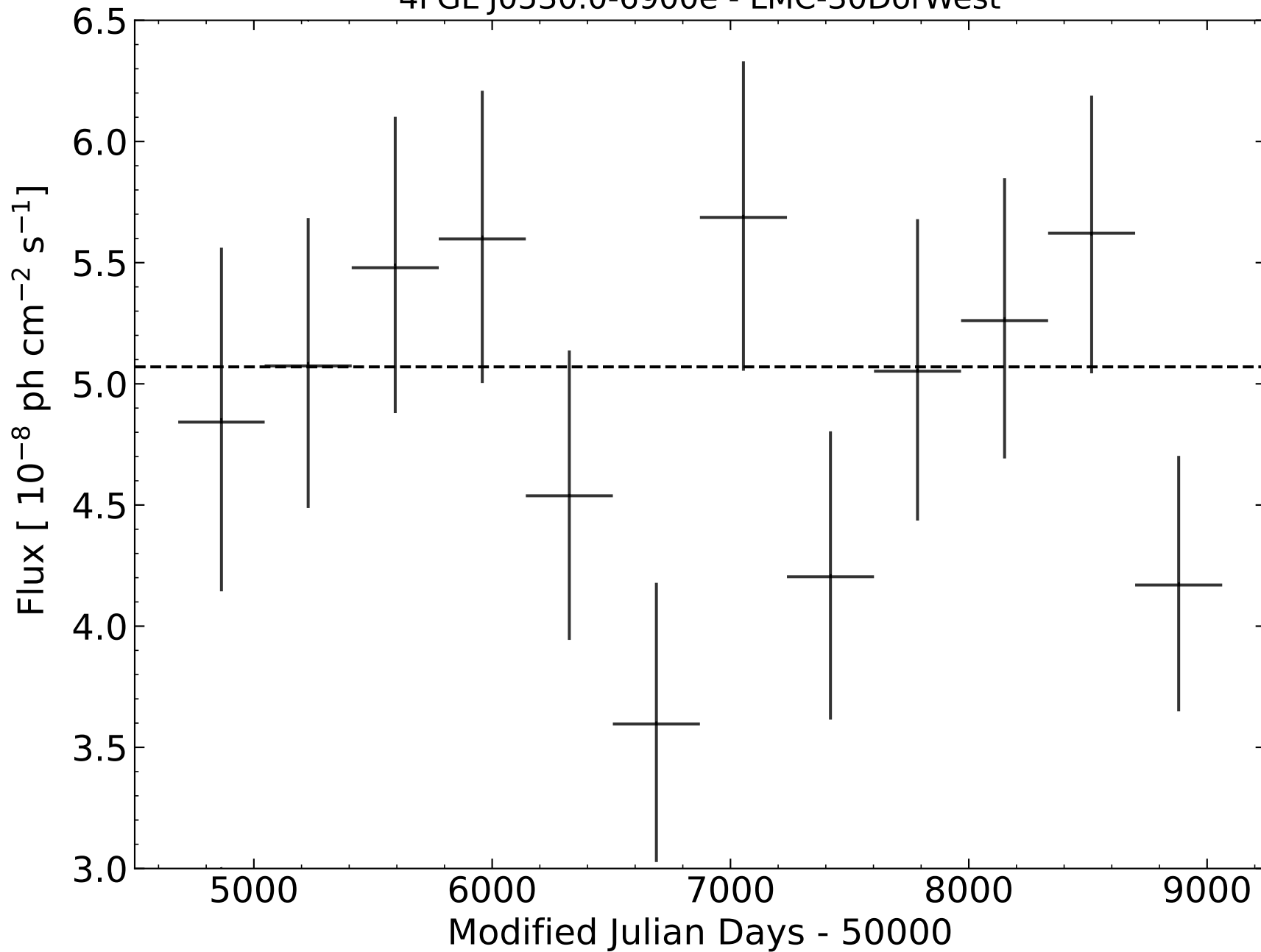
4FGL J0530.0-6900e - LMC-30DorWest
