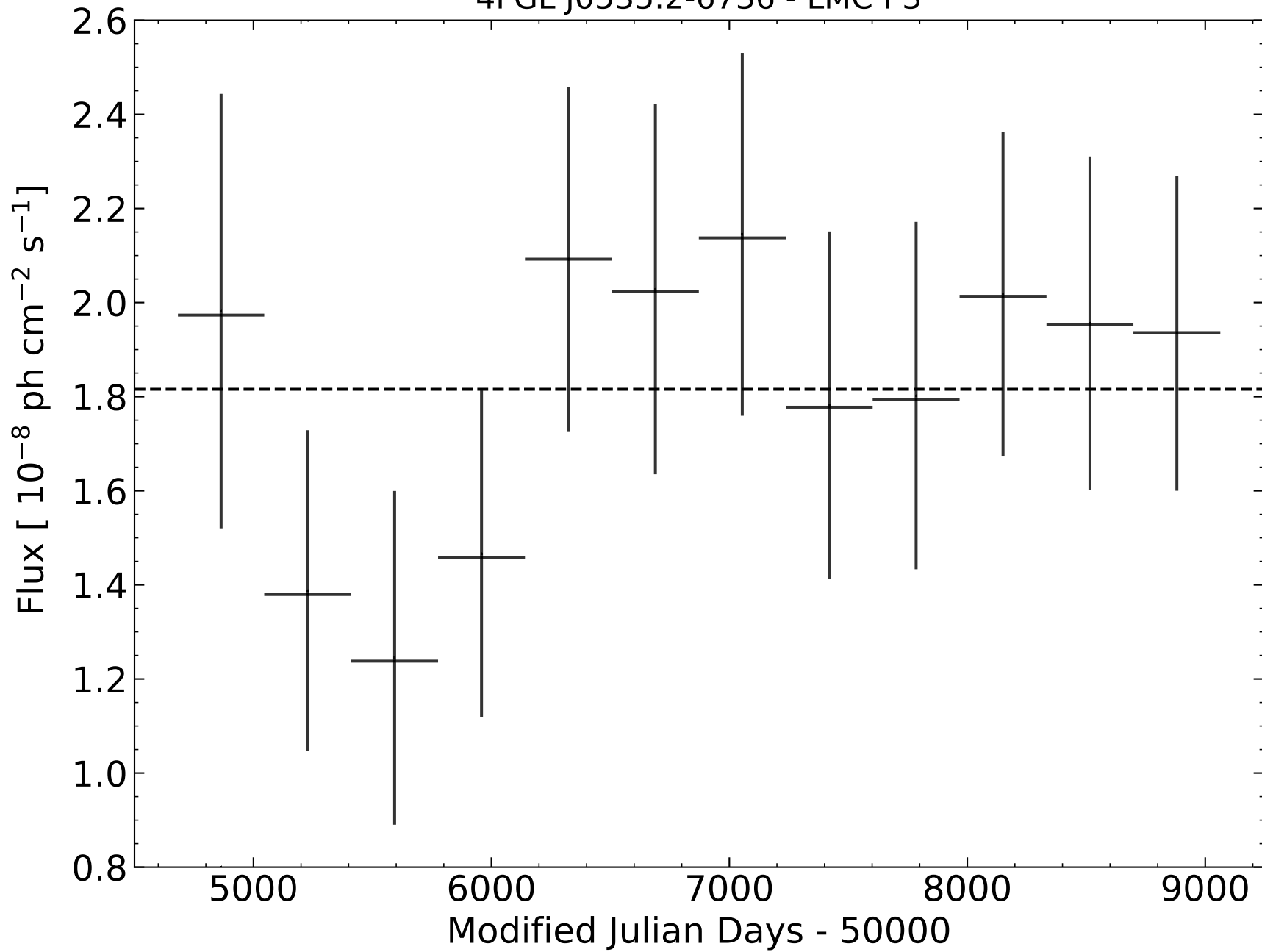
4FGL J0535.2-6736 - LMC P3
