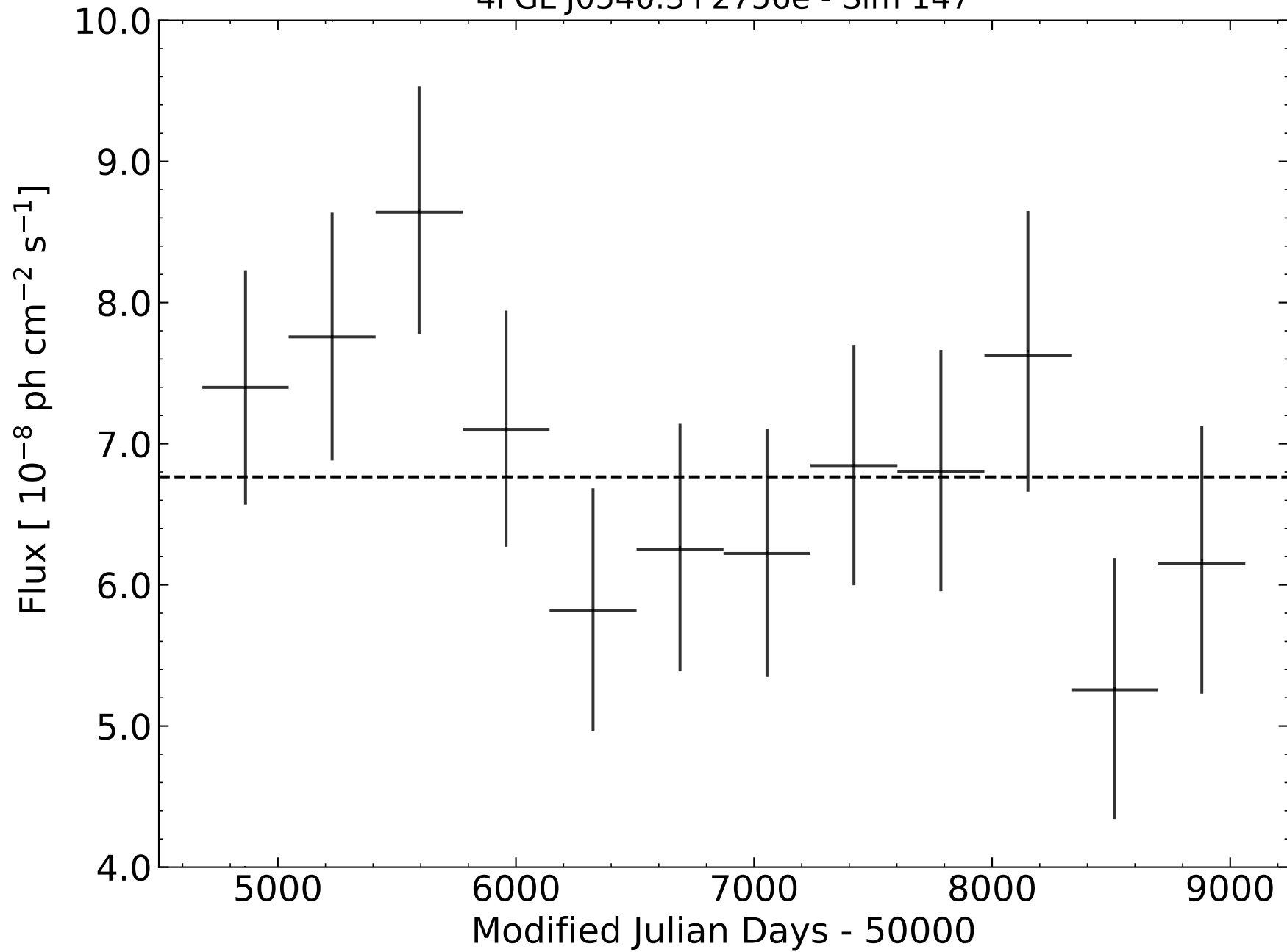
4FGL J0540.3+2756e - Sim 147
