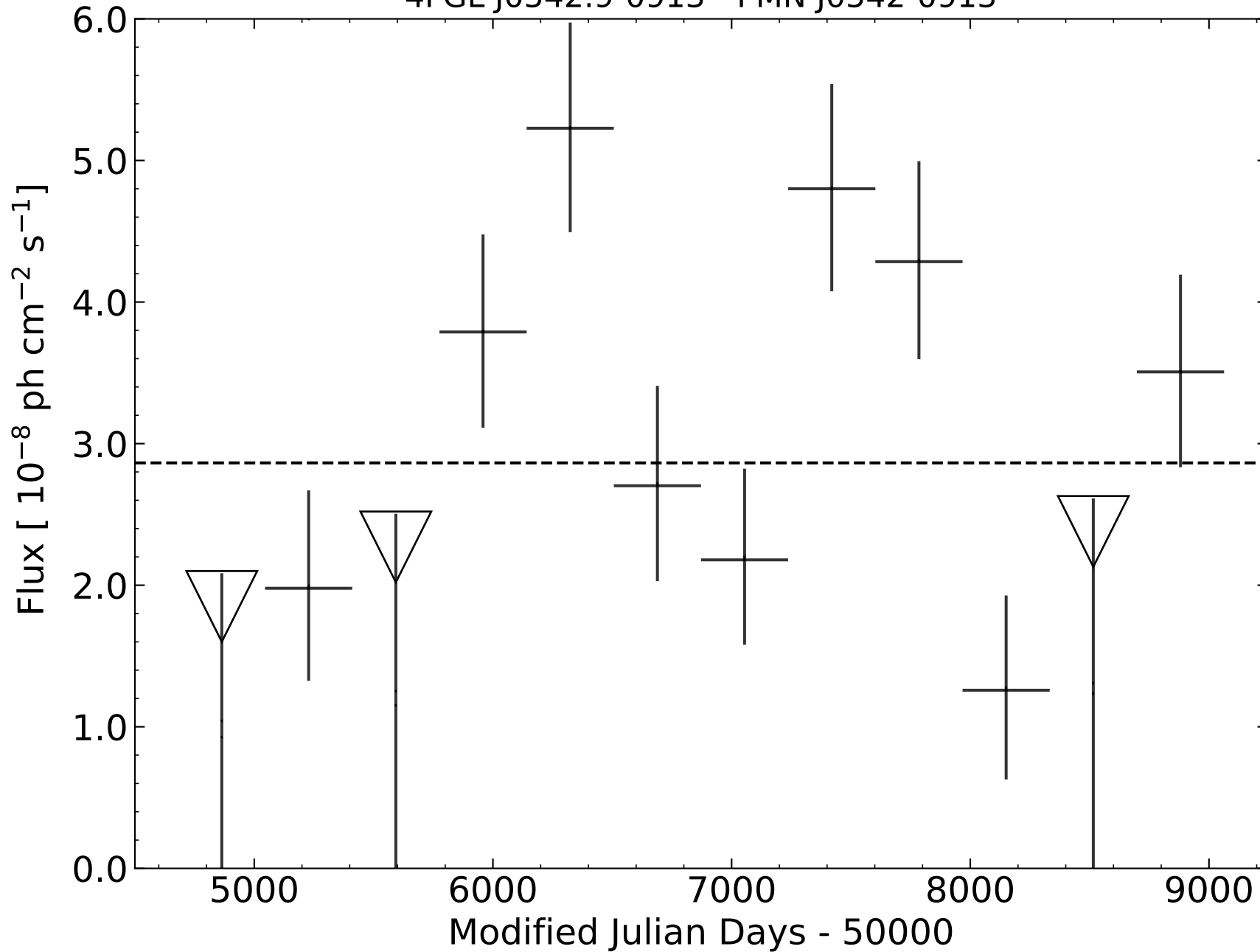
4FGL J0542.9-0913 - PMN J0542-0913
