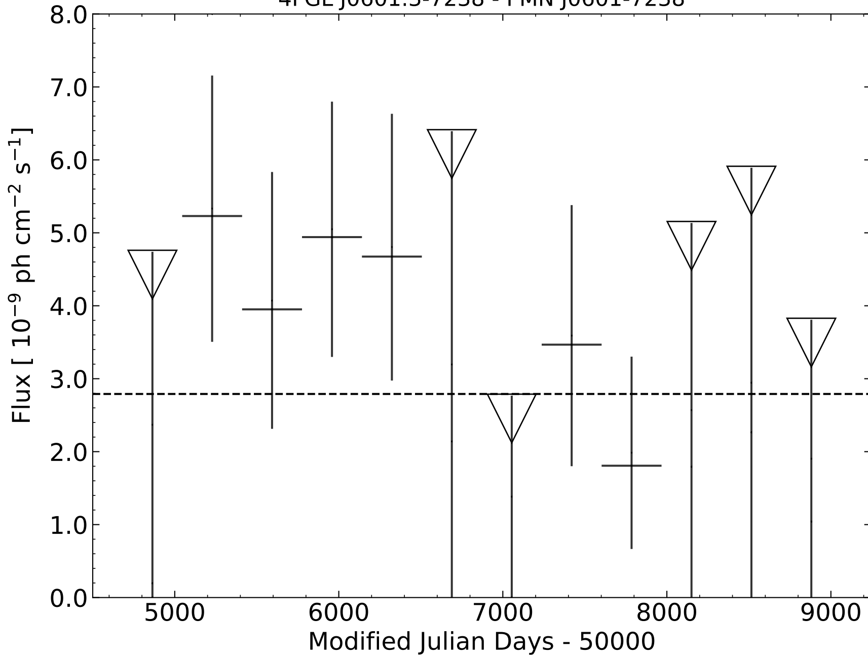
4FGL J0601.3-7238 - PMN J0601-7238
