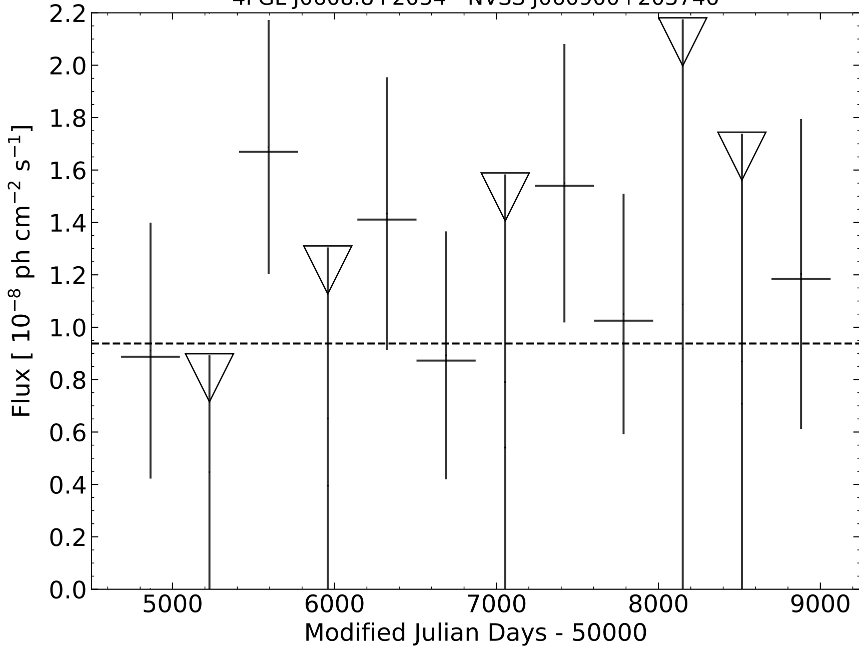
4FGL J0608.8+2034 - NVSS J060900+203746
