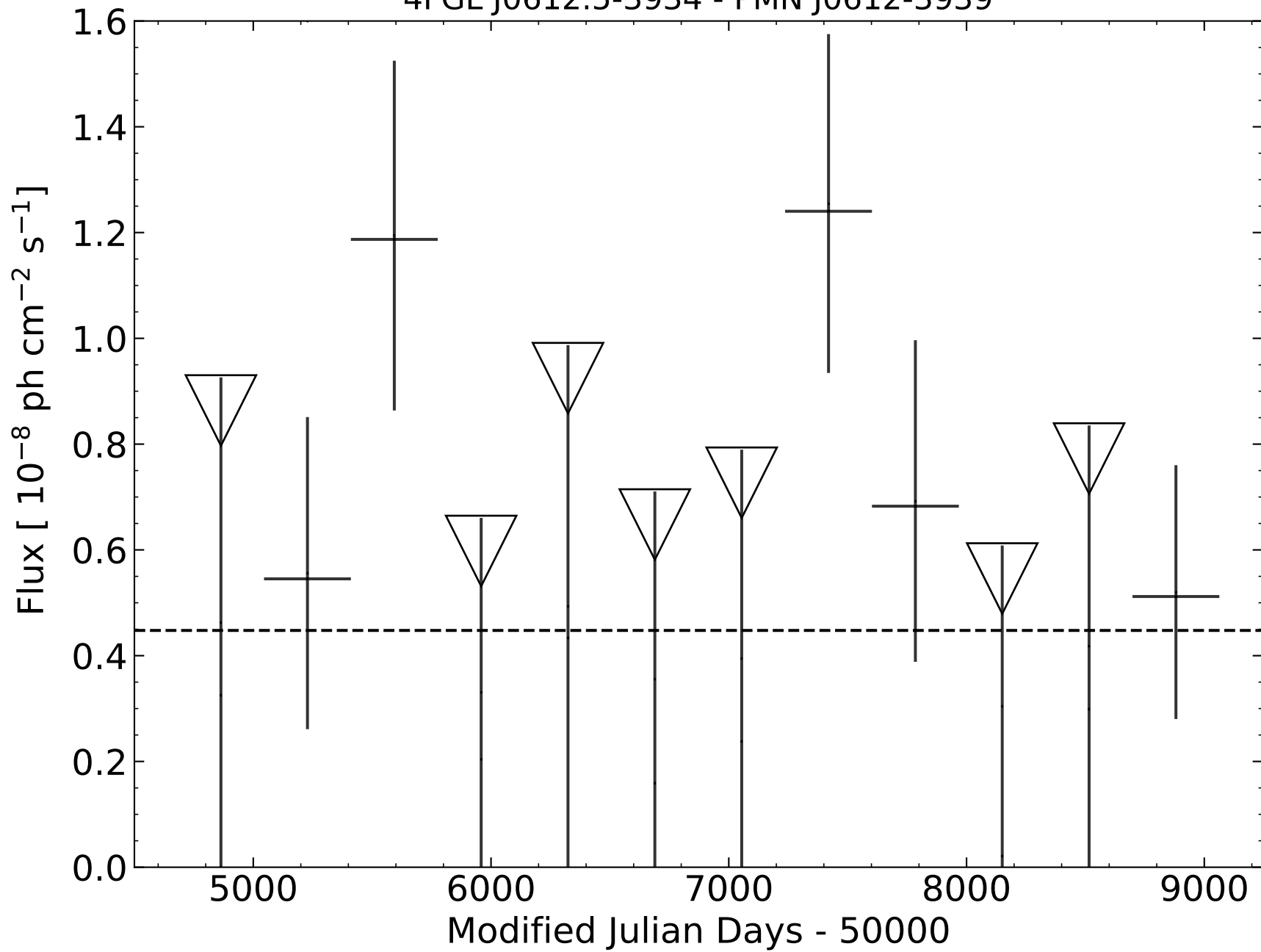
4FGL J0612.5-3934 - PMN J0612-3939
