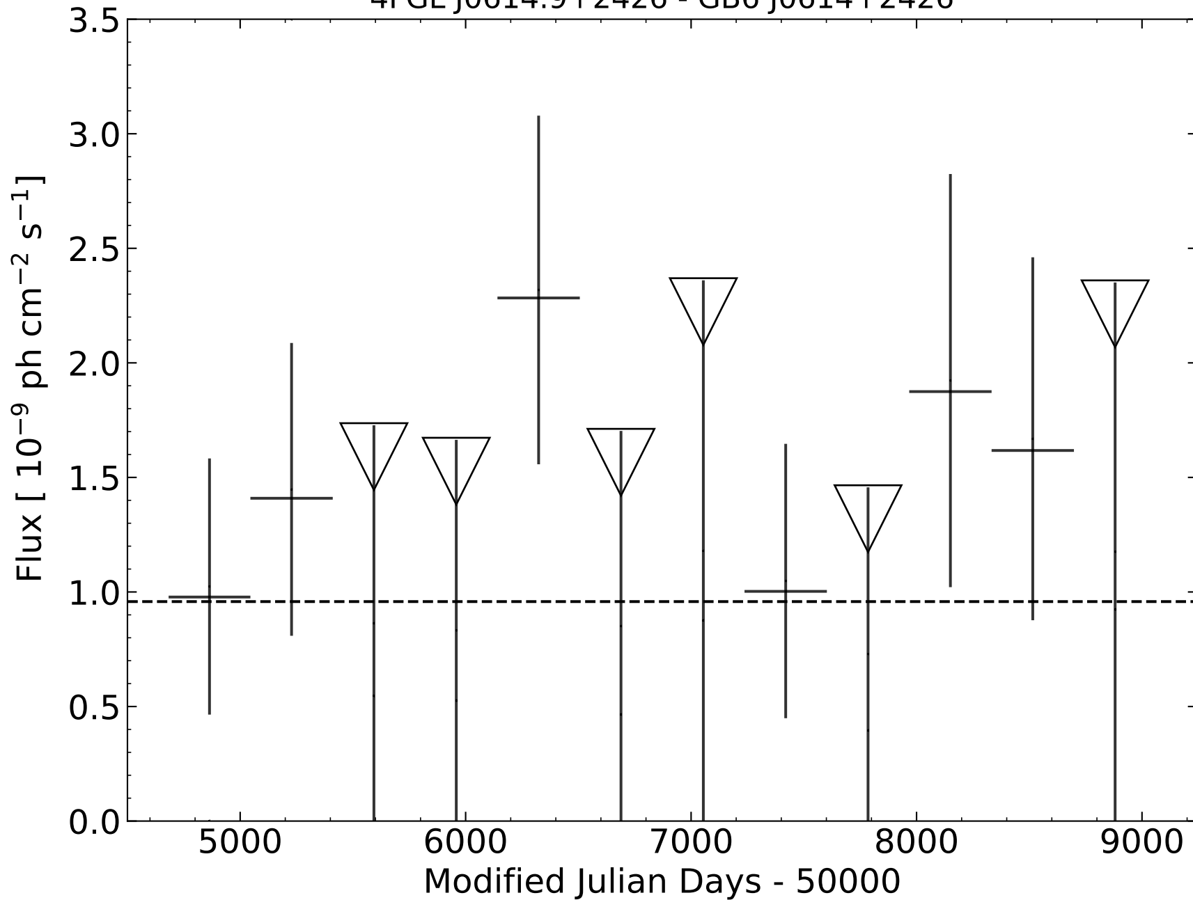
4FGL J0614.9+2426 - GB6 J0614+2426
