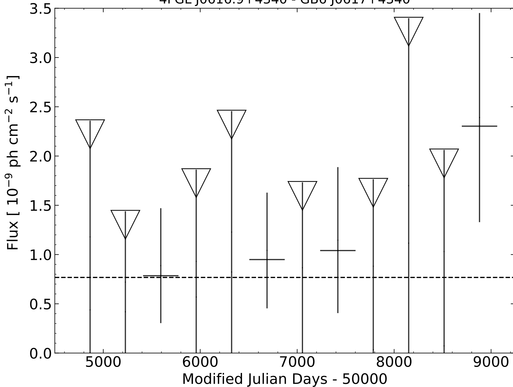
4FGL J0616.9+4340 - GB6 J0617+4340
