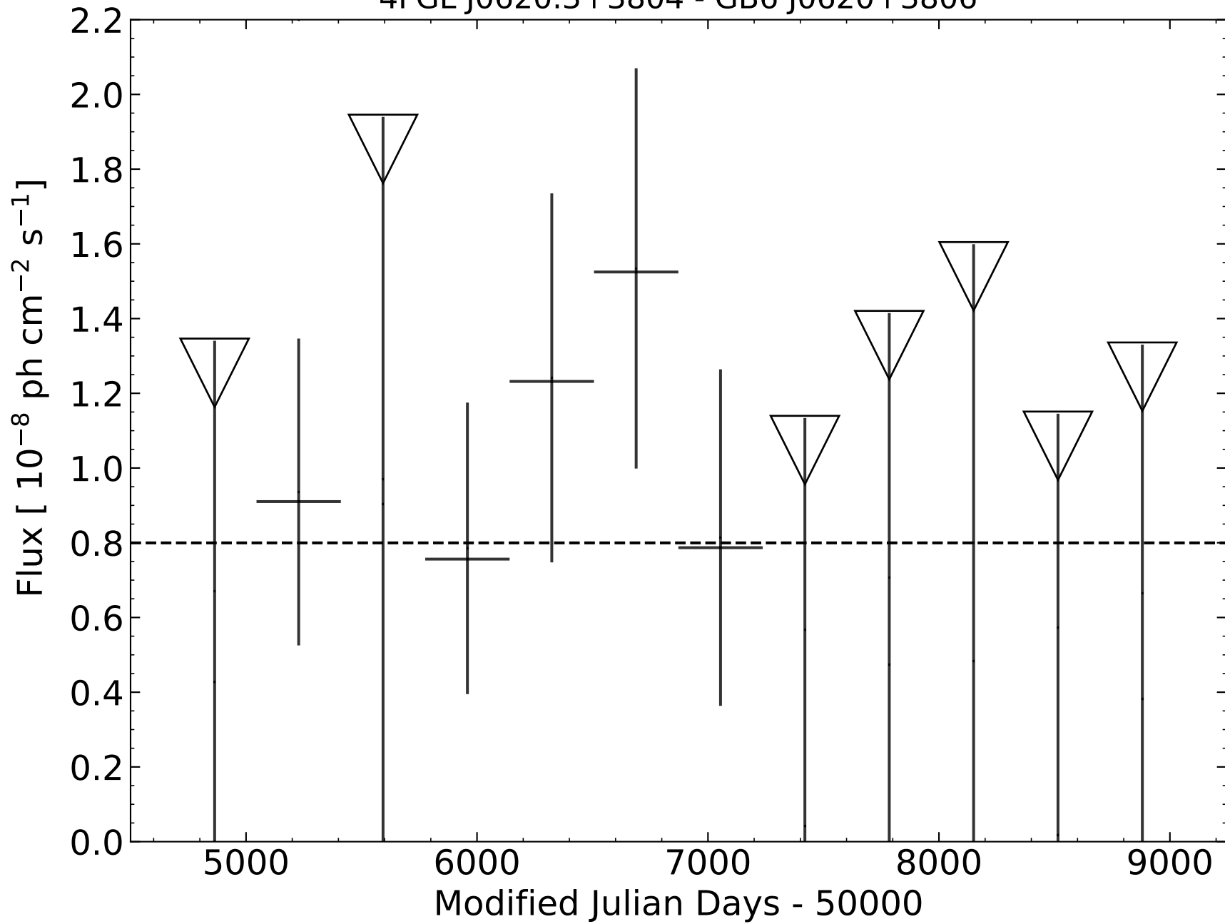
4FGL J0620.3+3804 - GB6 J0620+3806
