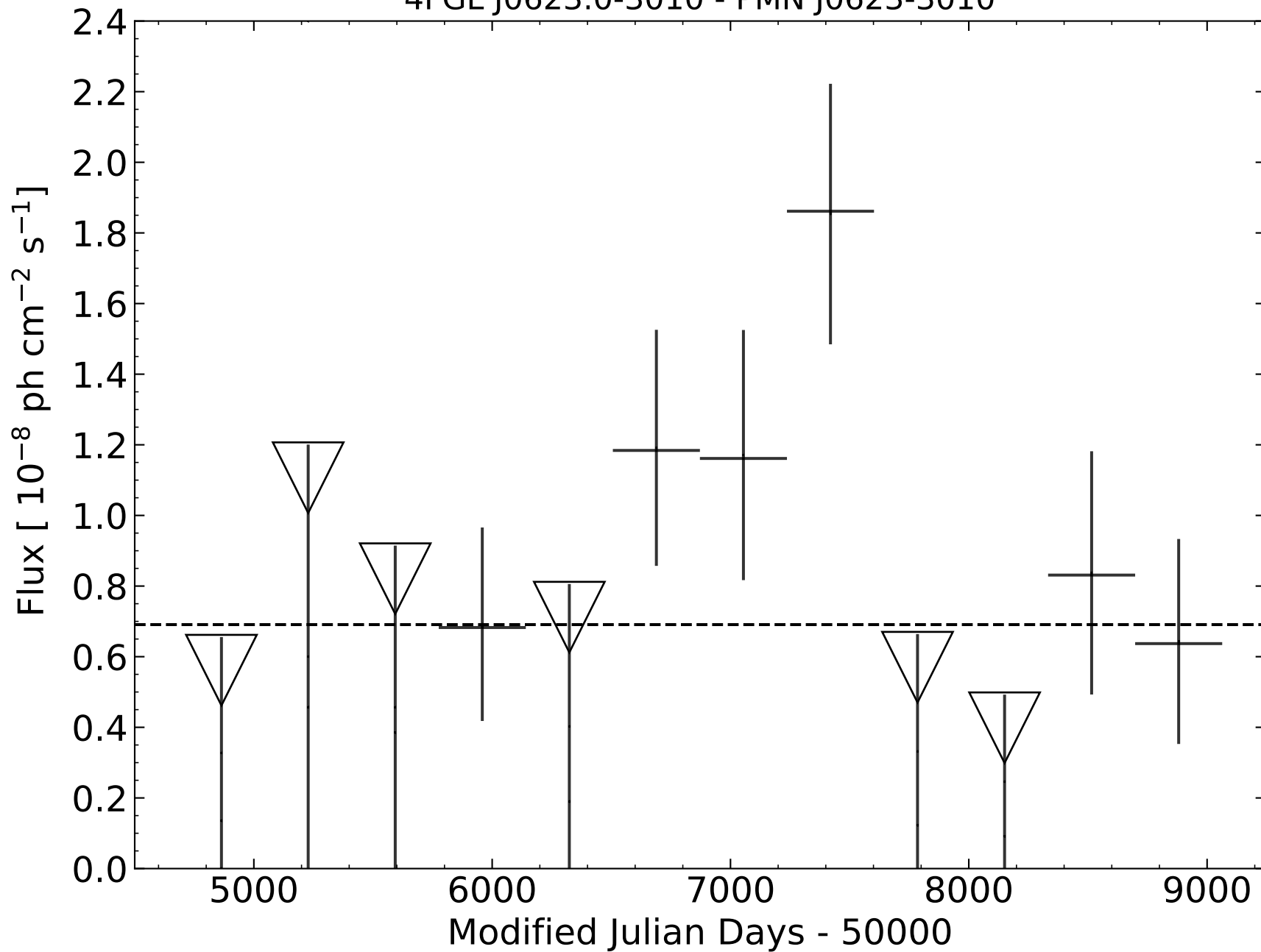
4FGL J0623.0-3010 - PMN J0623-3010
