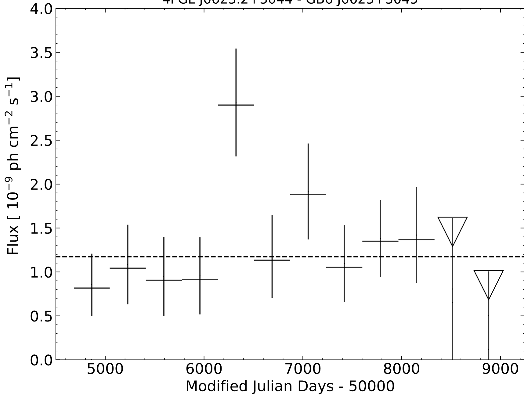
4FGL J0623.2+3044 - GB6 J0623+3045
