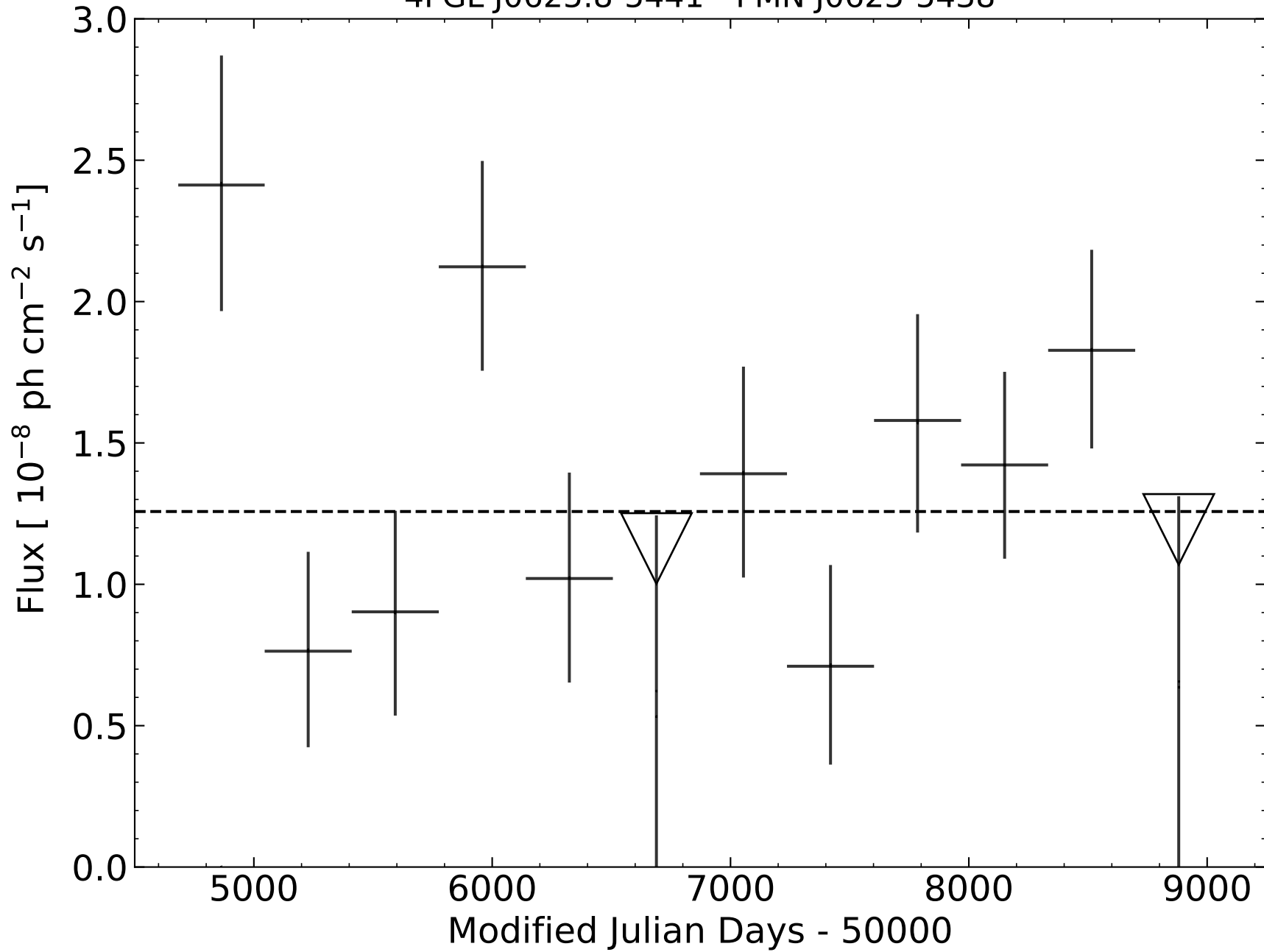
4FGL J0625.8-5441 - PMN J0625-5438
