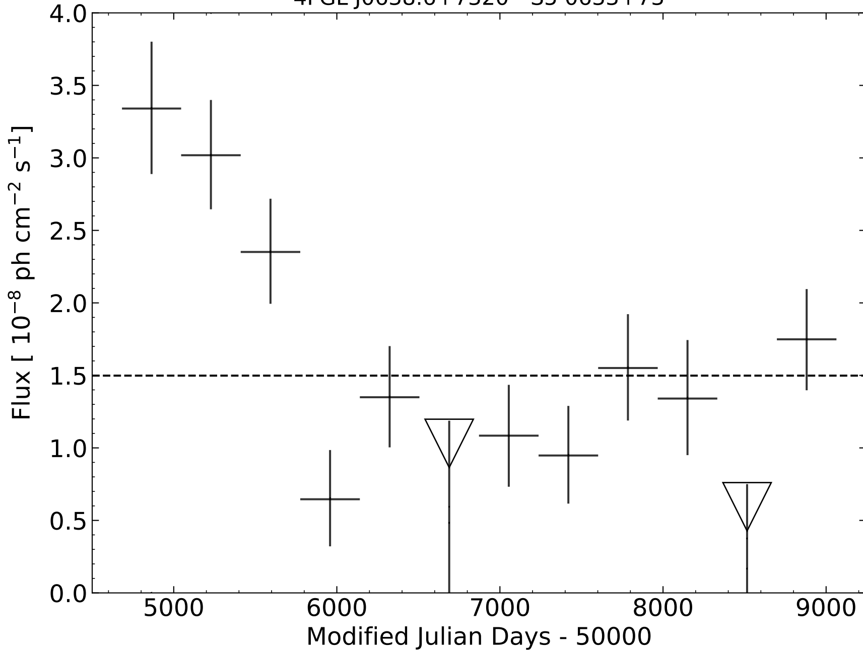
4FGL J0638.6+7320 - S5 0633+73
