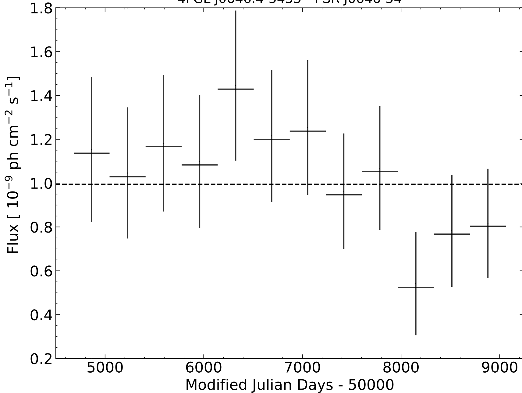
4FGL J0646.4-5455 - PSR J0646-54
