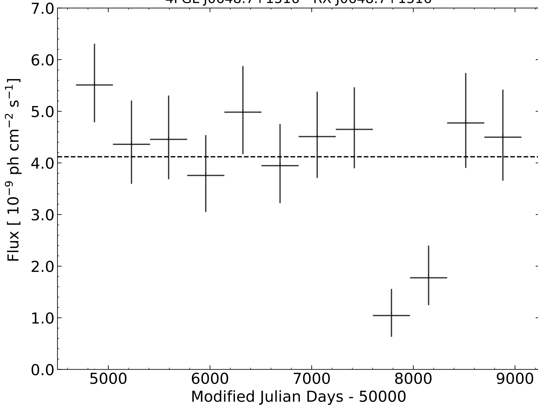
4FGL J0648.7+1516 - RX J0648.7+1516
