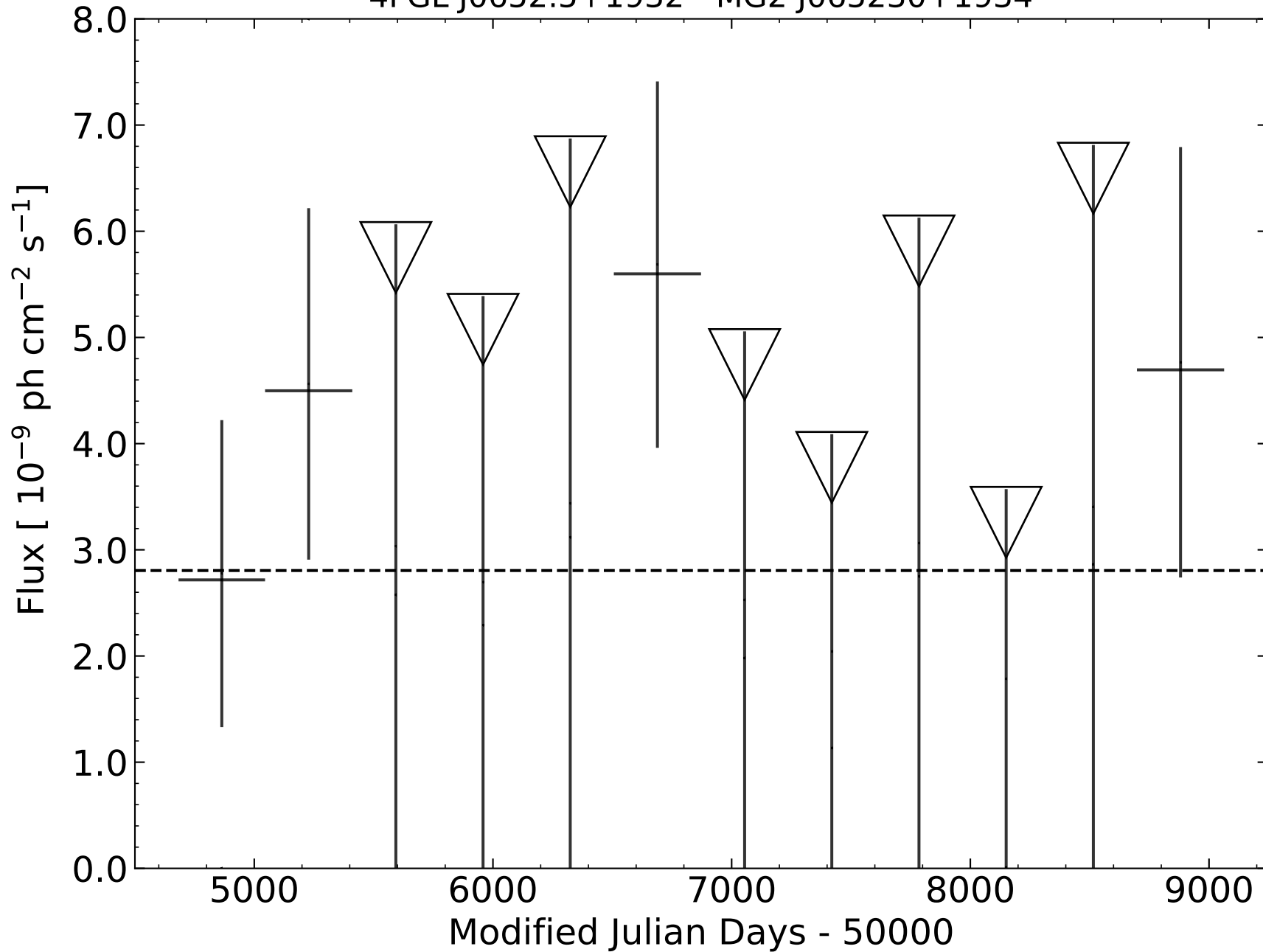
4FGL J0652.5+1932 - MG2 J065230+1934
