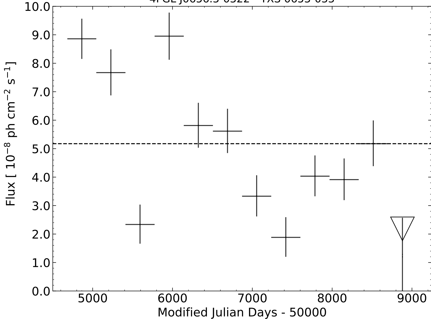
4FGL J0656.3-0322 - TXS 0653-033
