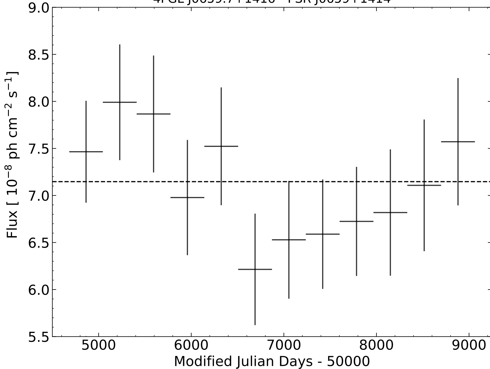
4FGL J0659.7+1416 - PSR J0659+1414
