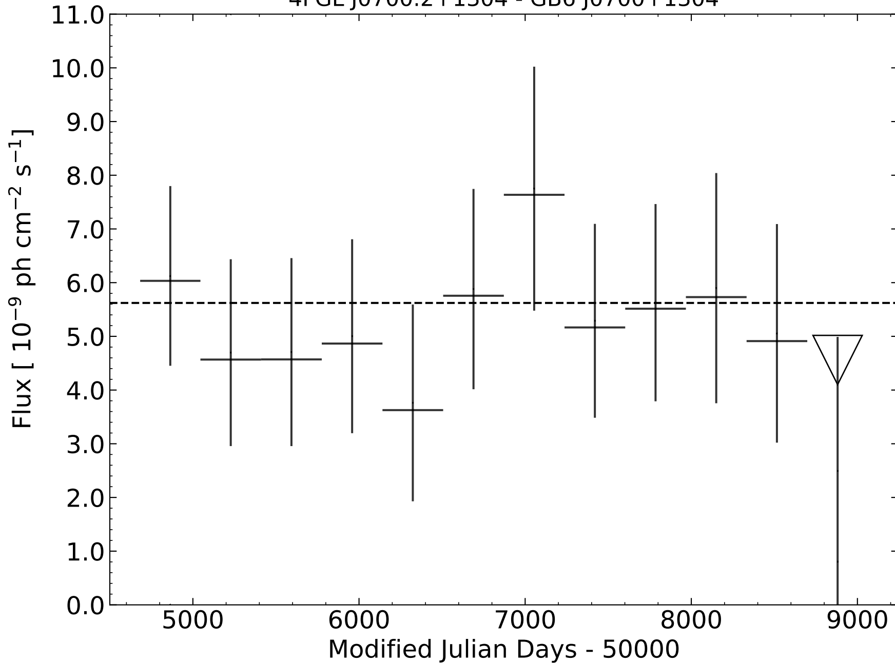
4FGL J0700.2+1304 - GB6 J0700+1304
