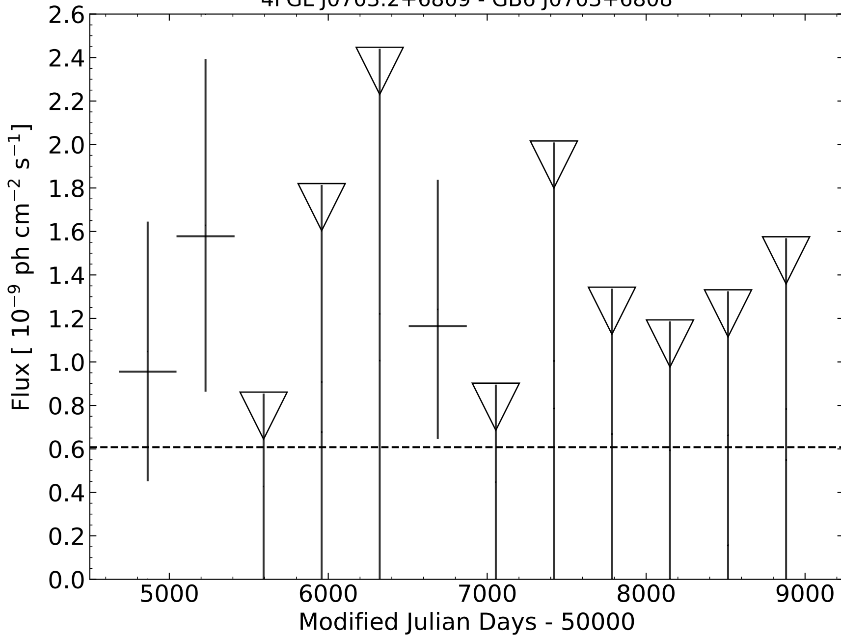
4FGL J0703.2+6809 - GB6 J0703+6808
