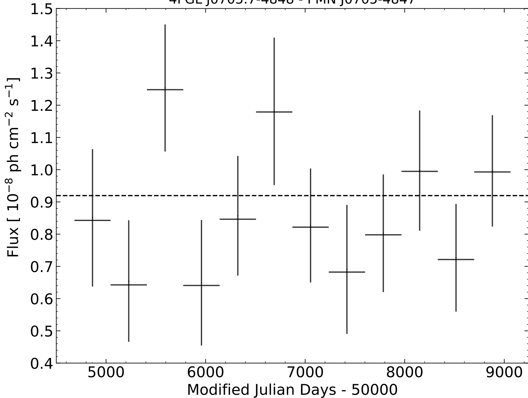
4FGL J0705.7-4848 - PMN J0705-4847
