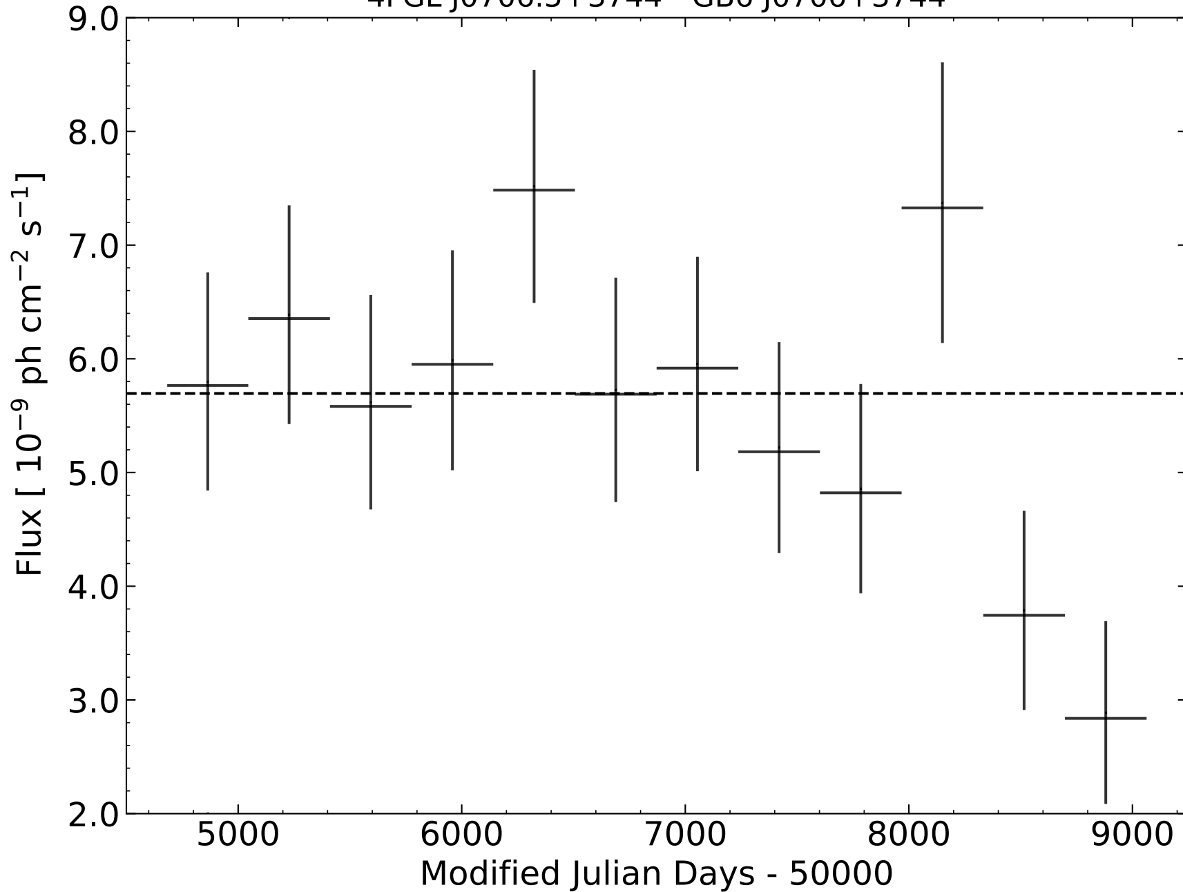
4FGL J0706.5+3744 - GB6 J0706+3744
