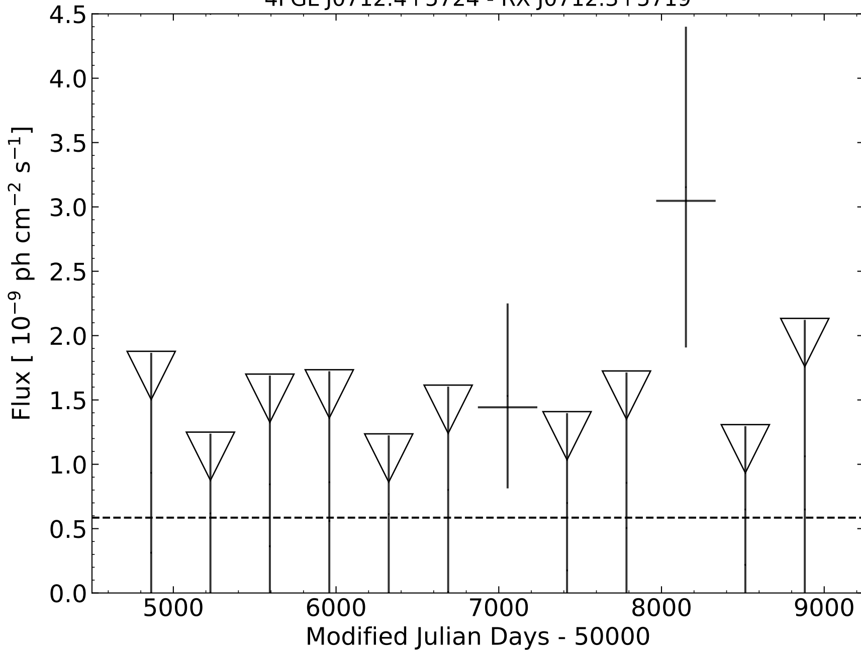
4FGL J0712.4+5724 - RX J0712.3+5719
