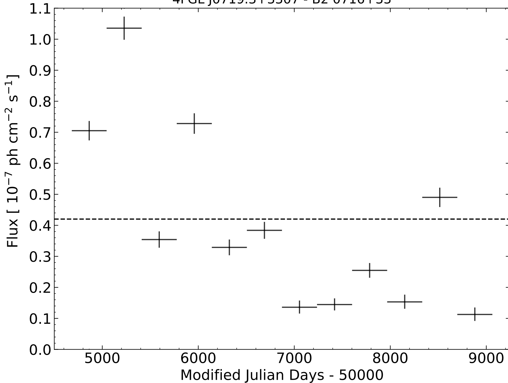
4FGL J0719.3+3307 - B2 0716+33
