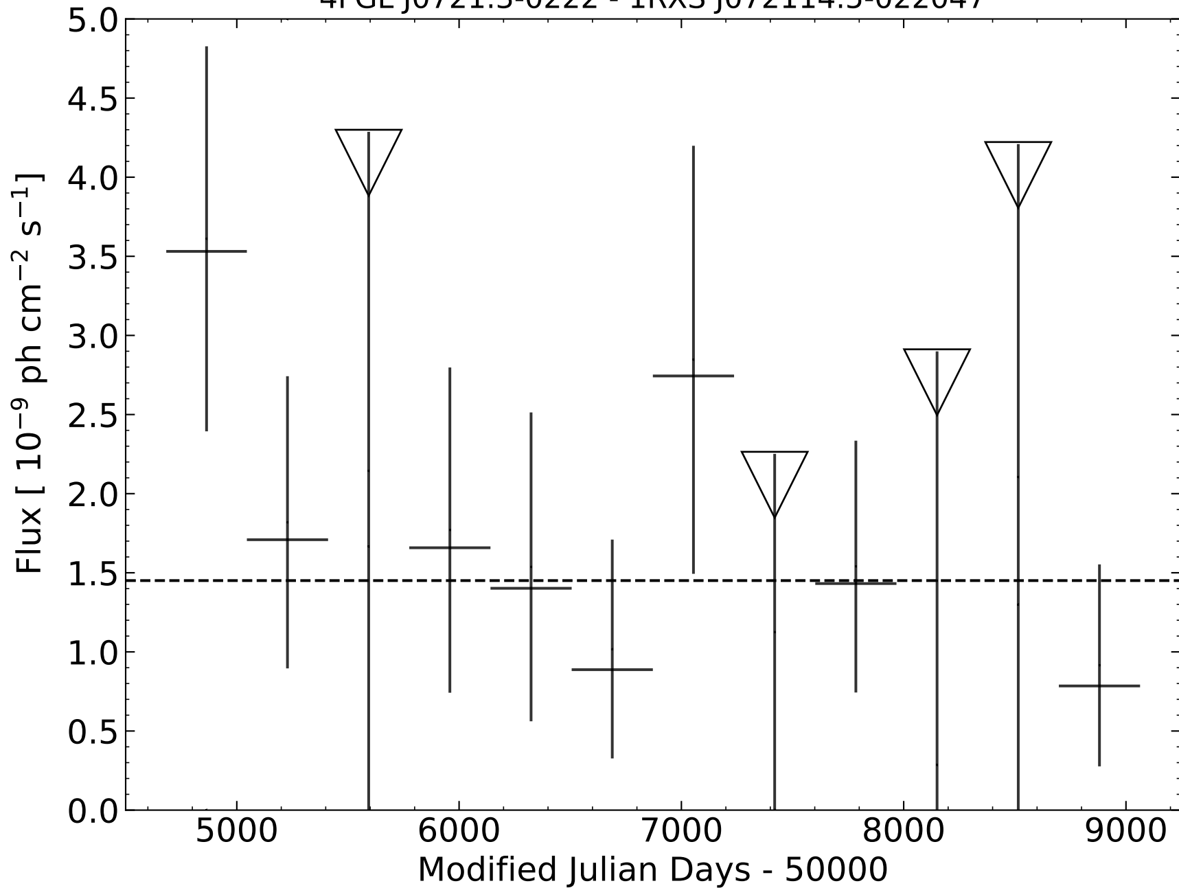
4FGL J0721.3-0222 - 1RXS J072114.5-022047
