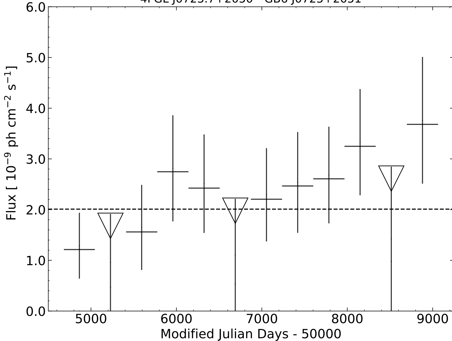
4FGL J0723.7+2050 - GB6 J0723+2051
