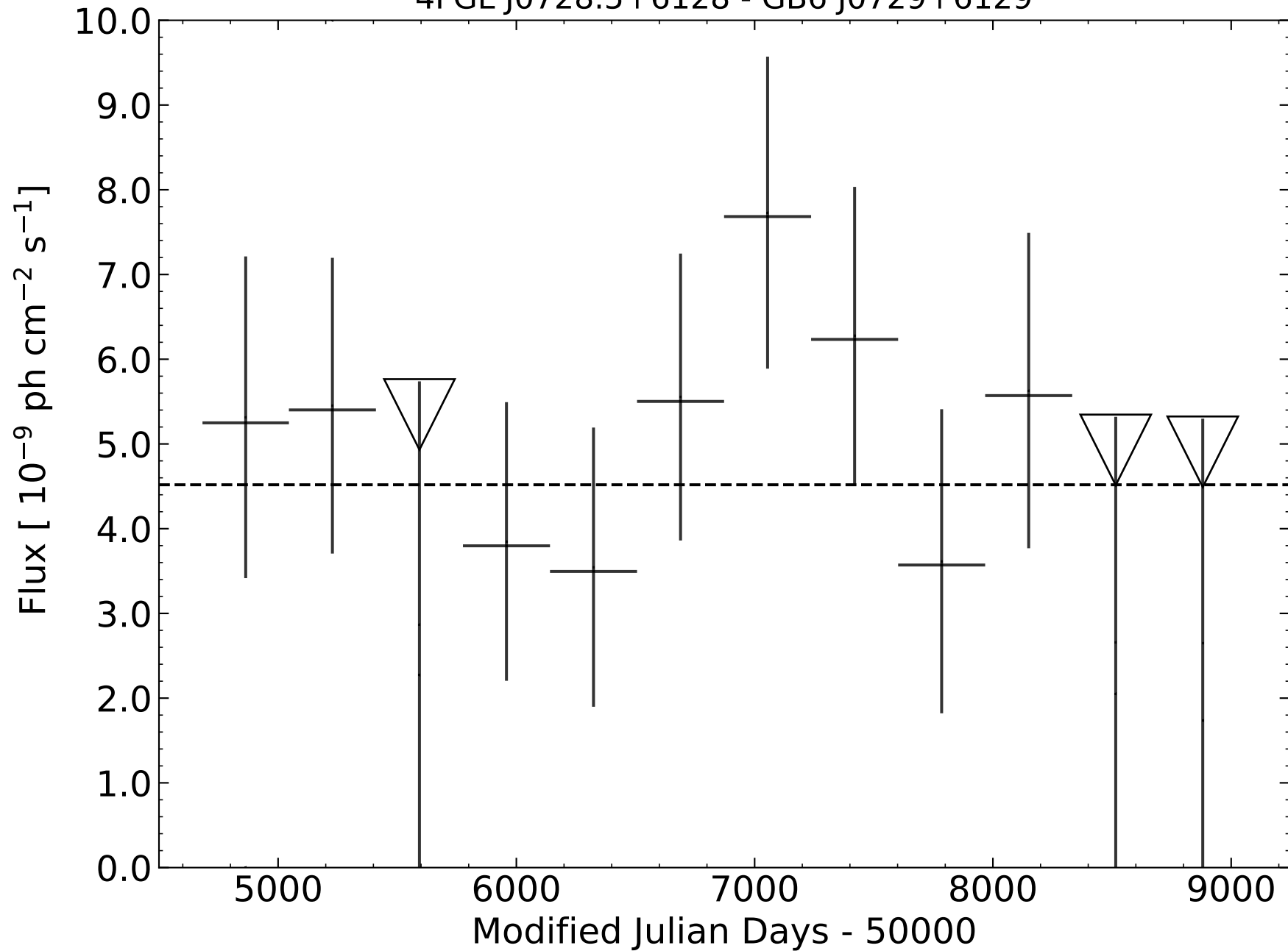
4FGL J0728.5+6128 - GB6 J0729+6129
