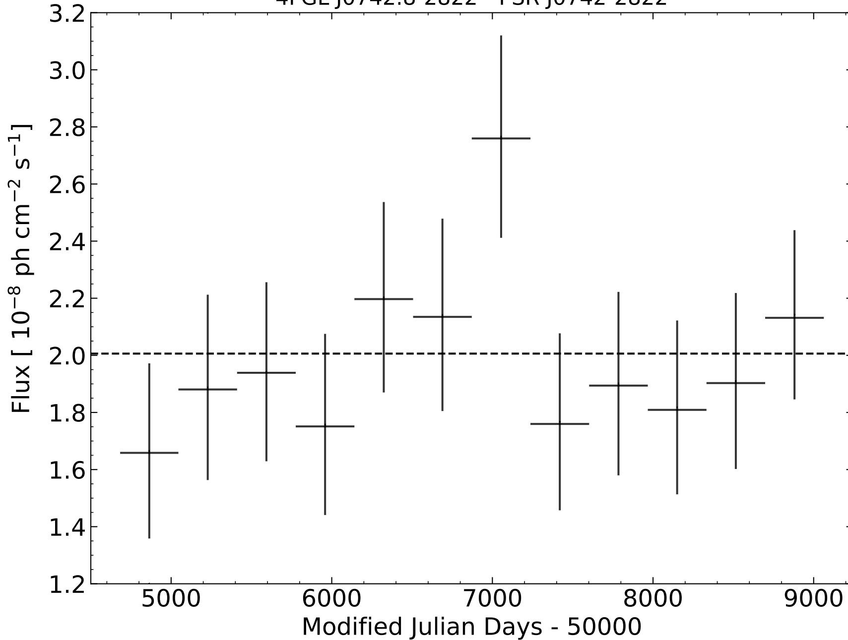
4FGL J0742.8-2822 - PSR J0742-2822
