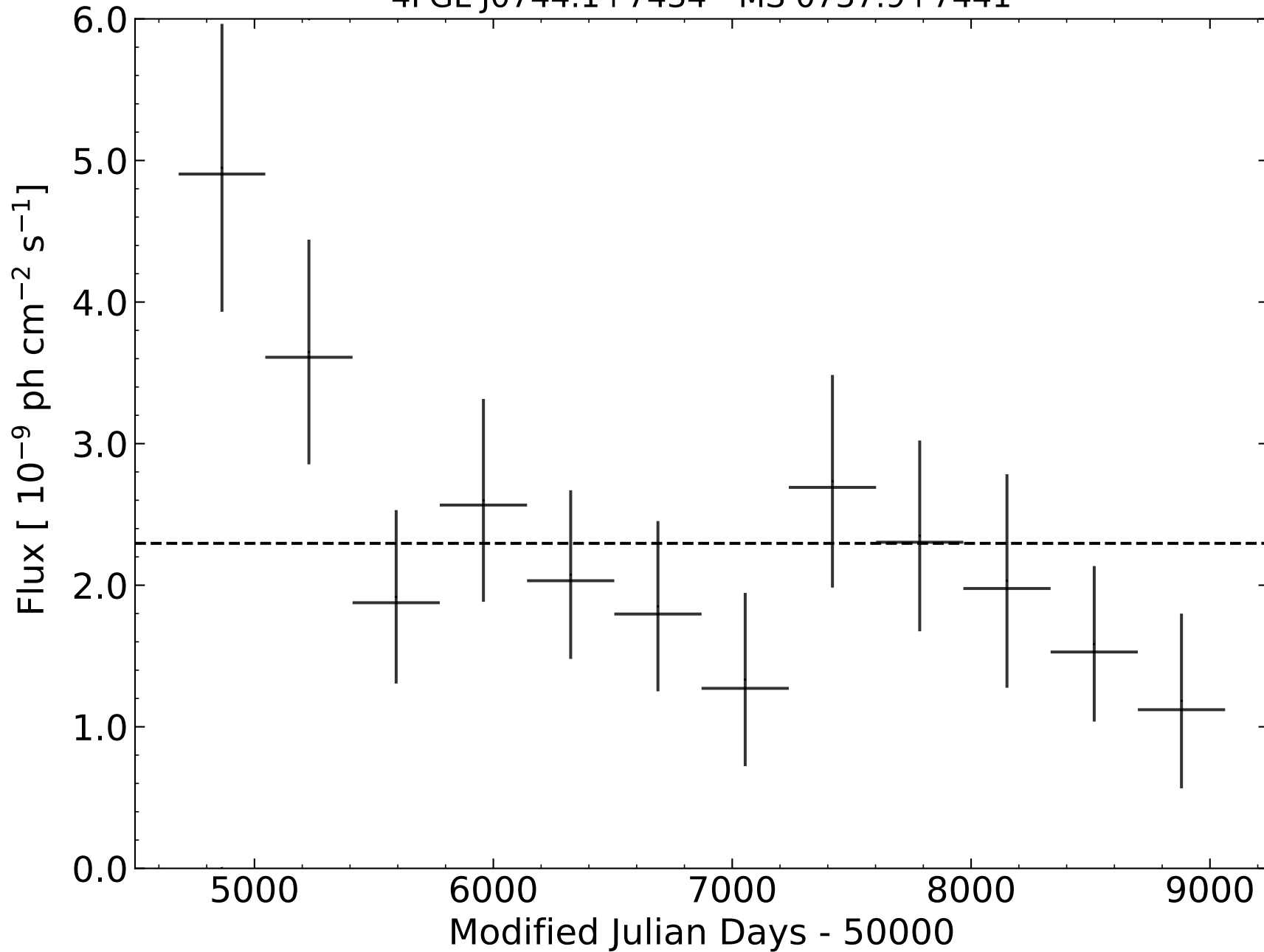
4FGL J0744.1+7434 - MS 0737.9+7441
