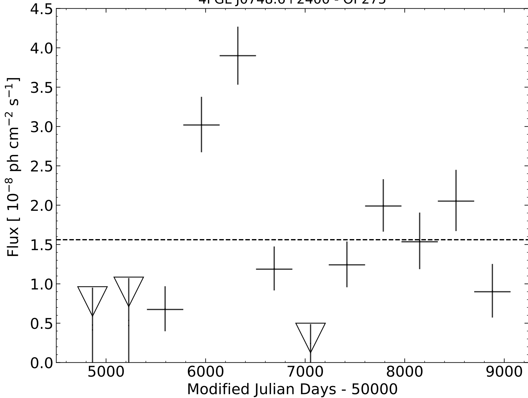
4FGL J0748.6+2400 - OI 275
