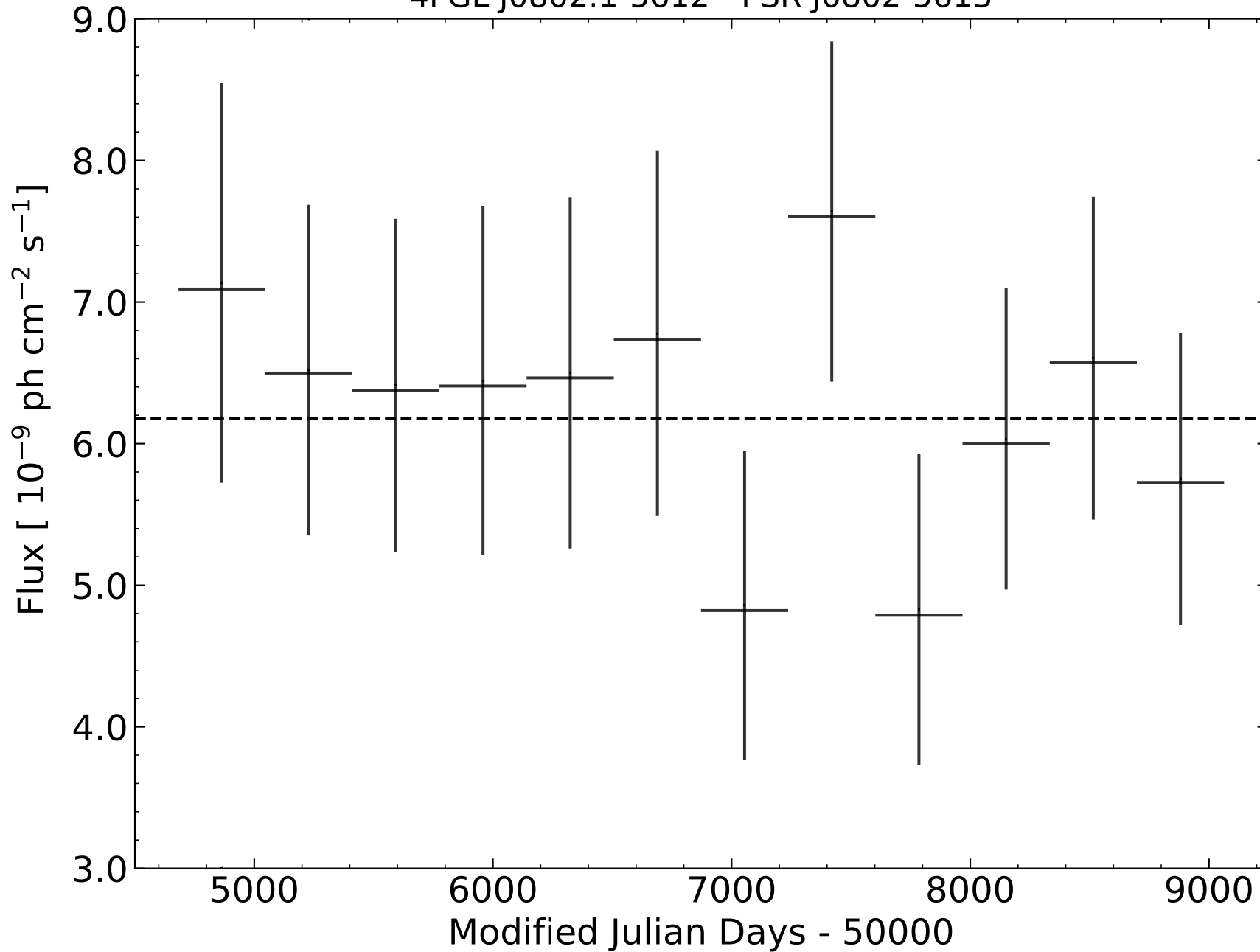
4FGL J0802.1-5612 - PSR J0802-5613
