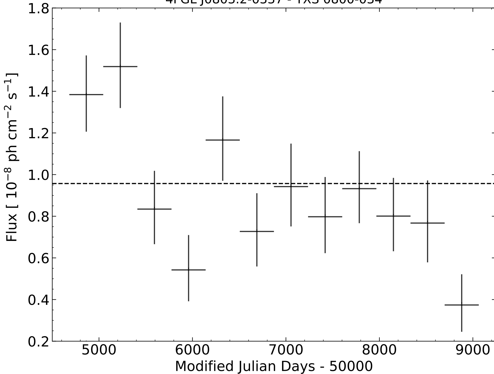
4FGL J0803.2-0337 - TXS 0800-034
