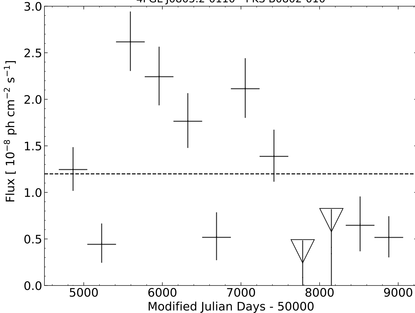
4FGL J0805.2-0110 - PKS B0802-010
