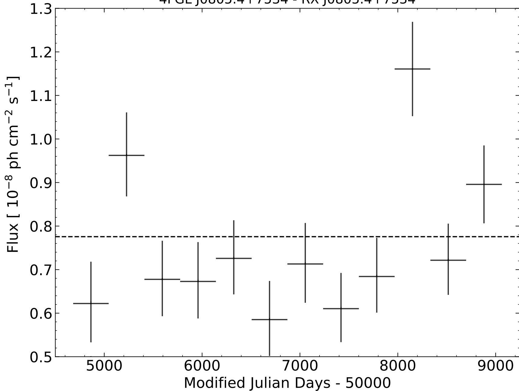
4FGL J0805.4+7534 - RX J0805.4+7534
