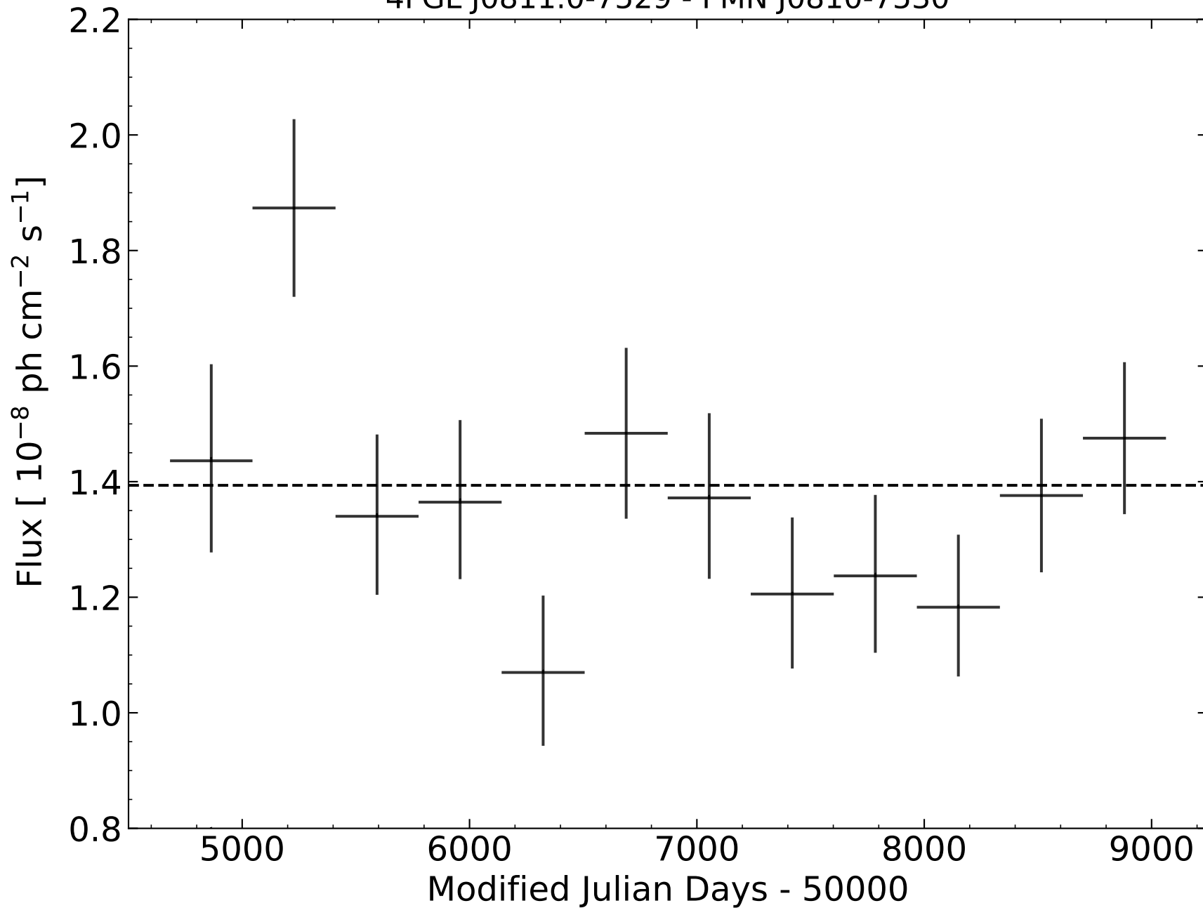
4FGL J0811.0-7529 - PMN J0810-7530
