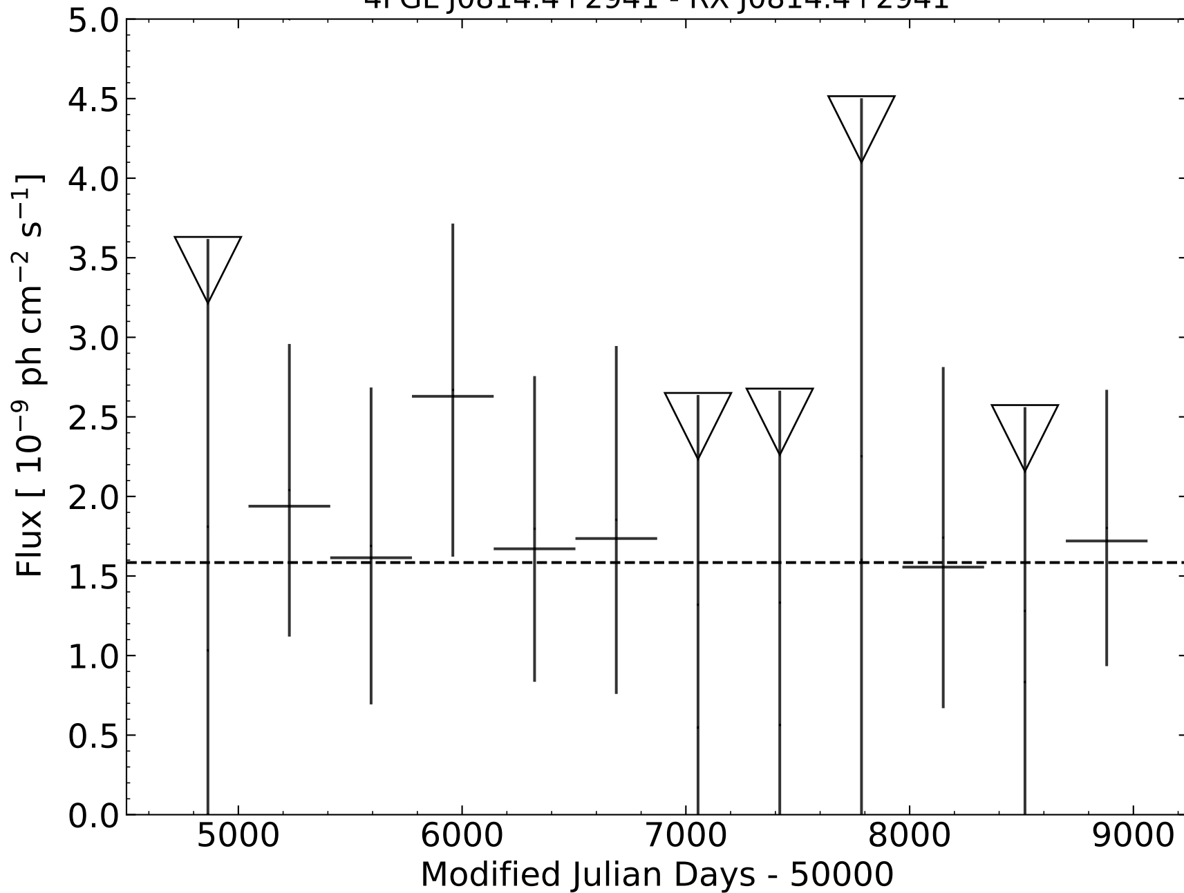
4FGL J0814.4+2941 - RX J0814.4+2941
