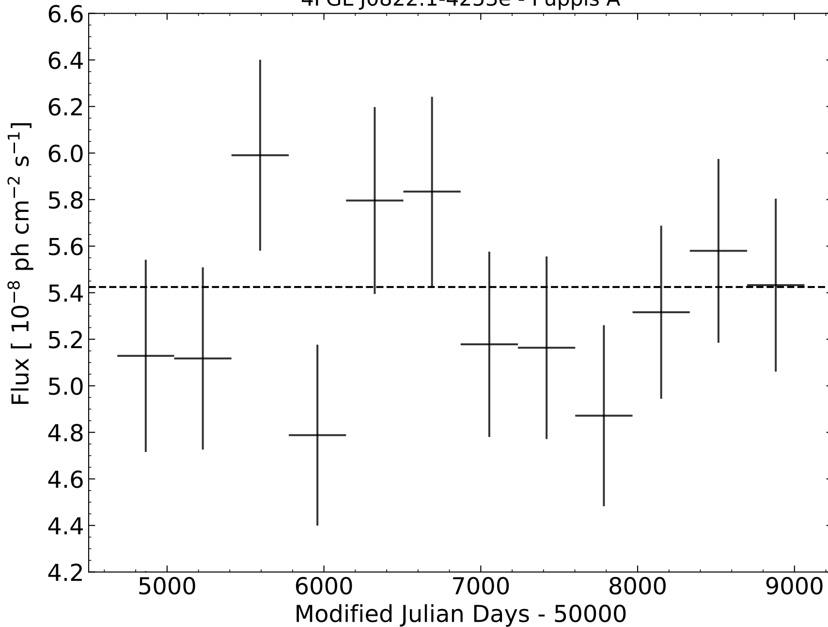
4FGL J0822.1-4253e - Puppis A
