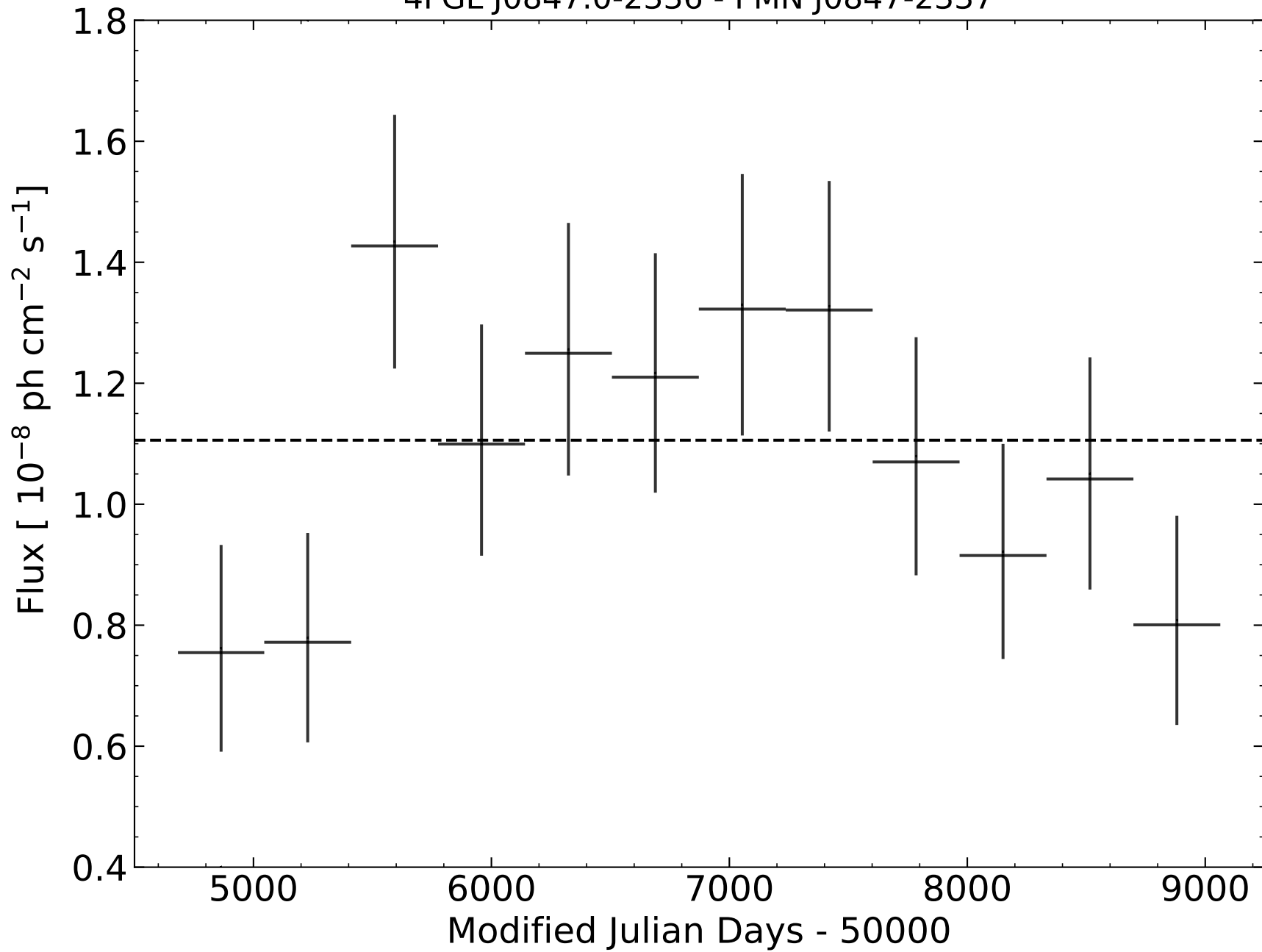
4FGL J0847.0-2336 - PMN J0847-2337
