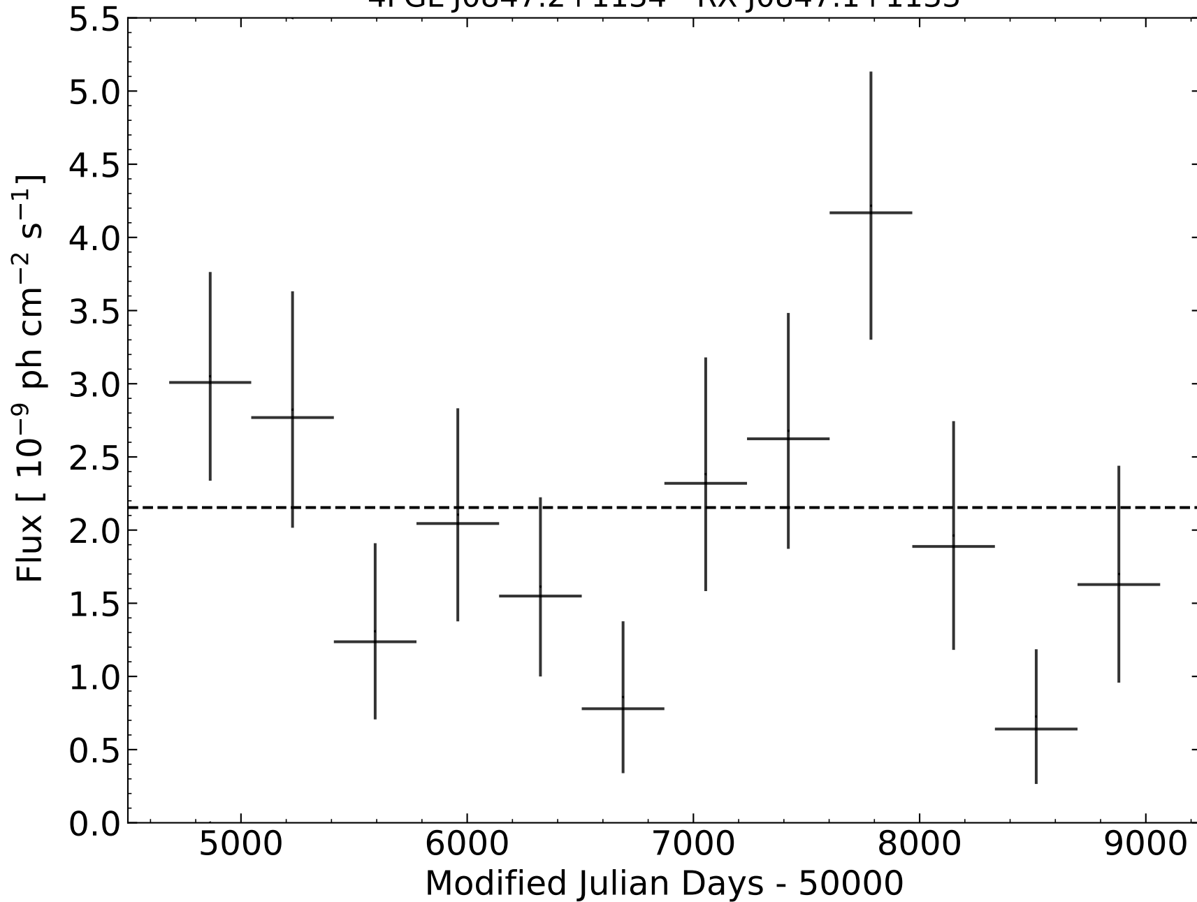
4FGL J0847.2+1134 - RX J0847.1+1133
