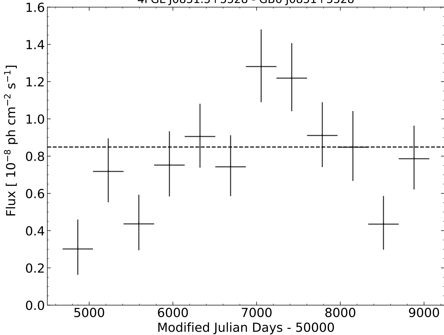
4FGL J0851.5+5528 - GB6 J0851+5528
