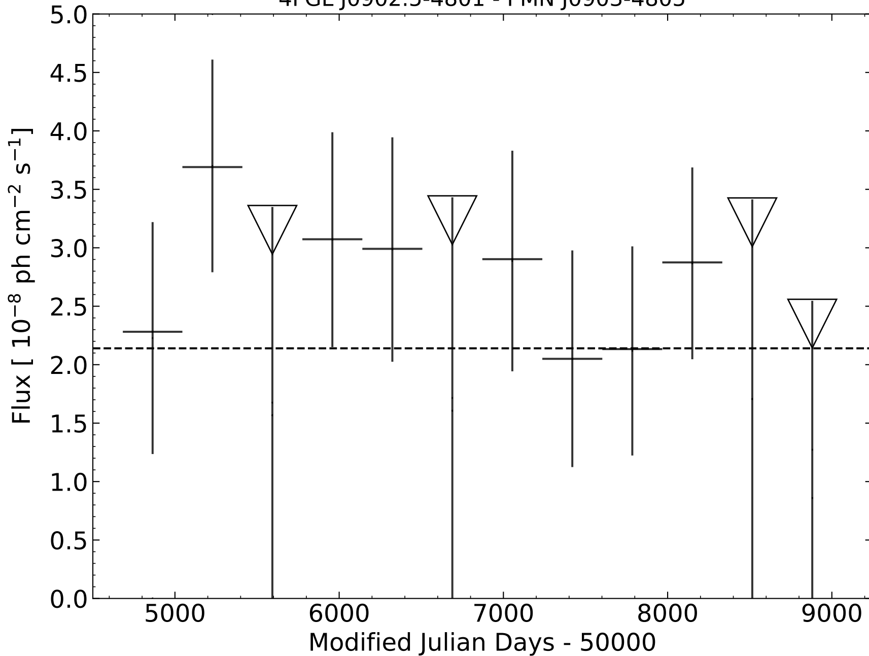
4FGL J0902.5-4801 - PMN J0903-4805
