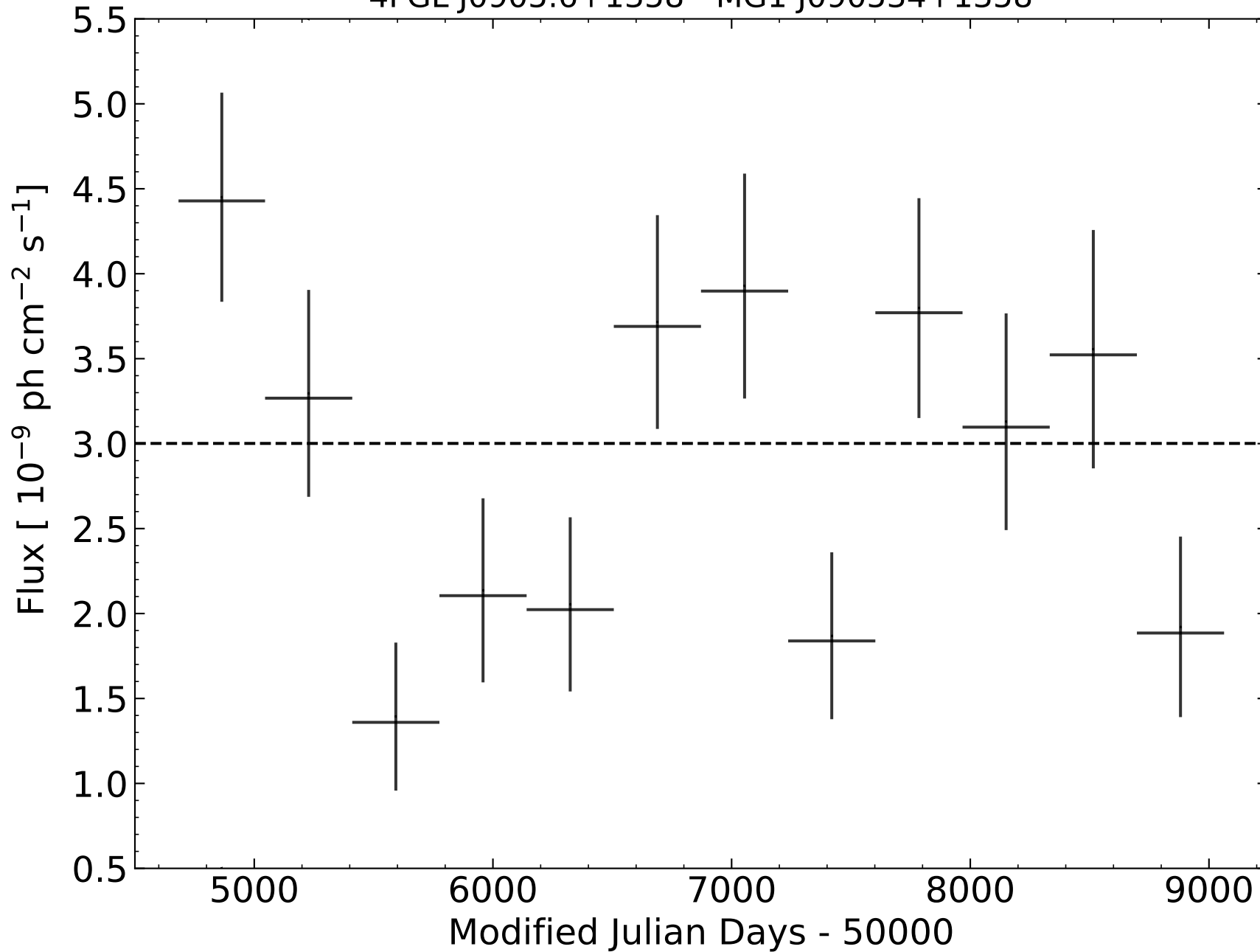
4FGL J0905.6+1358 - MG1 J090534+1358
