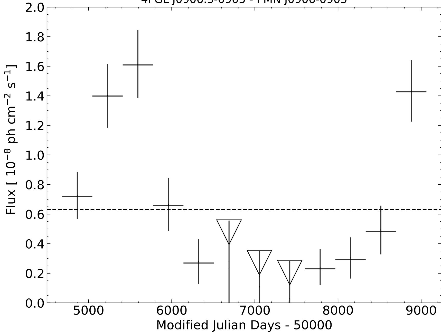
4FGL J0906.3-0905 - PMN J0906-0905
