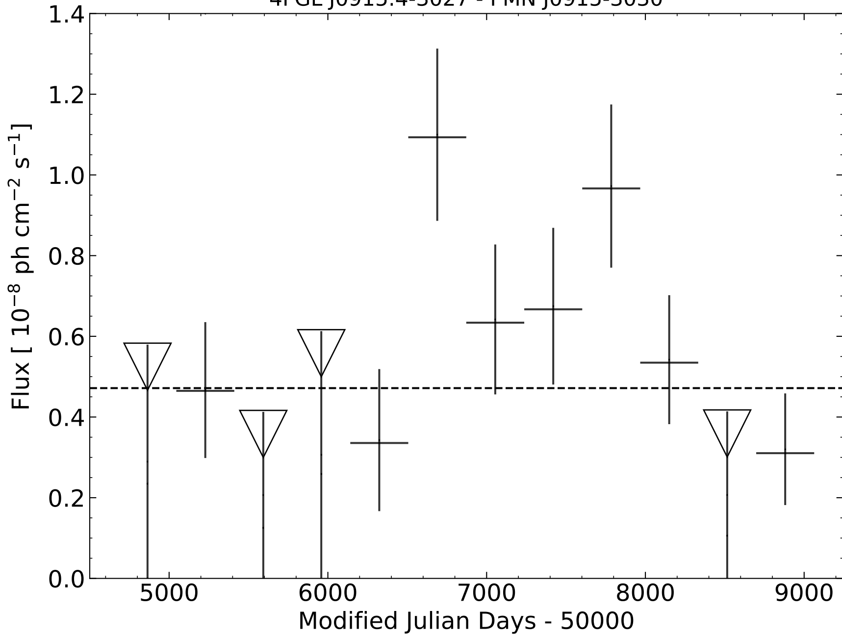
4FGL J0915.4-3027 - PMN J0915-3030
