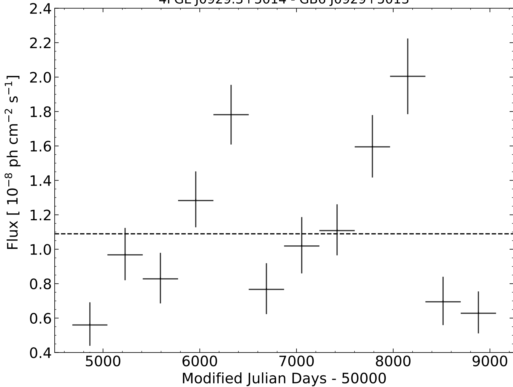
4FGL J0929.3+5014 - GB6 J0929+5013
