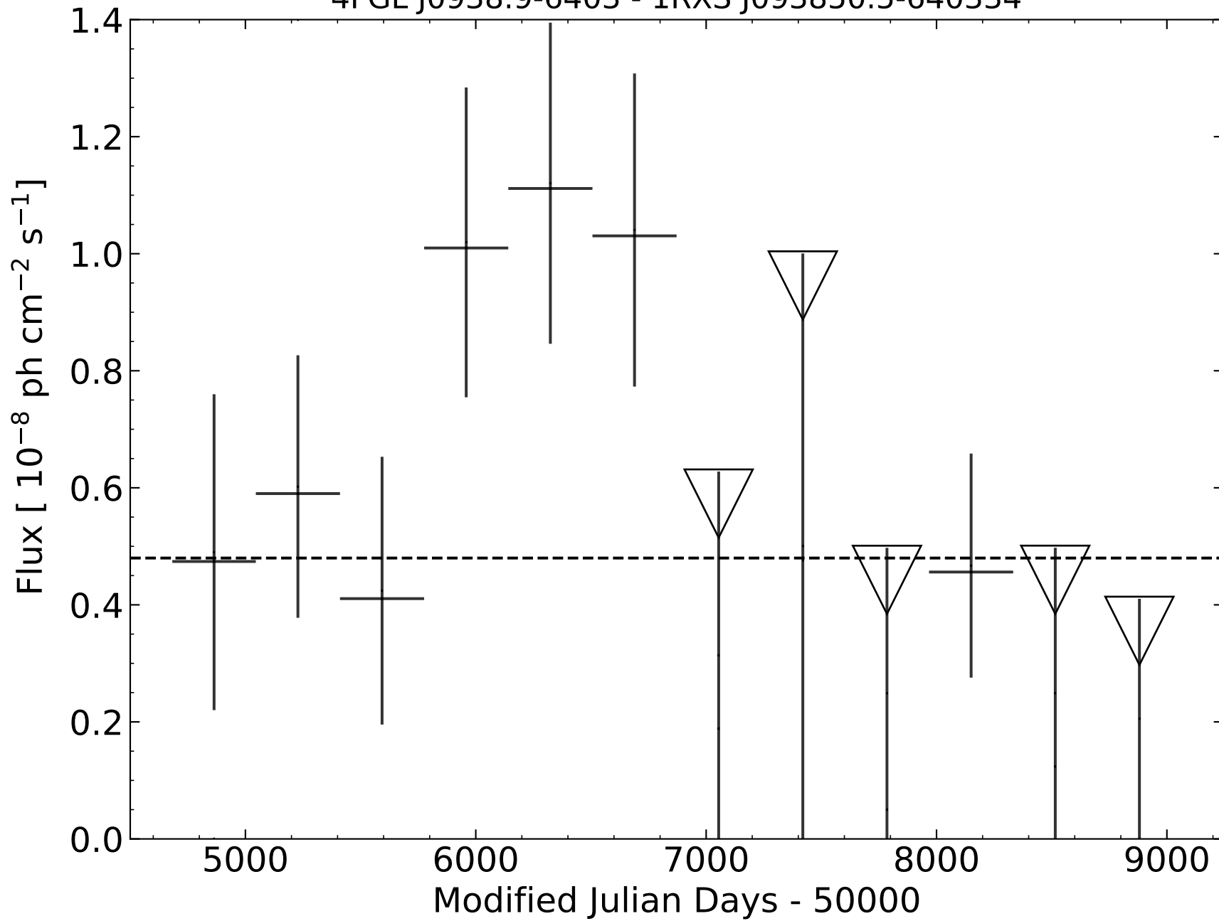
4FGL J0938.9-6403 - 1RXS J093850.5-640334
