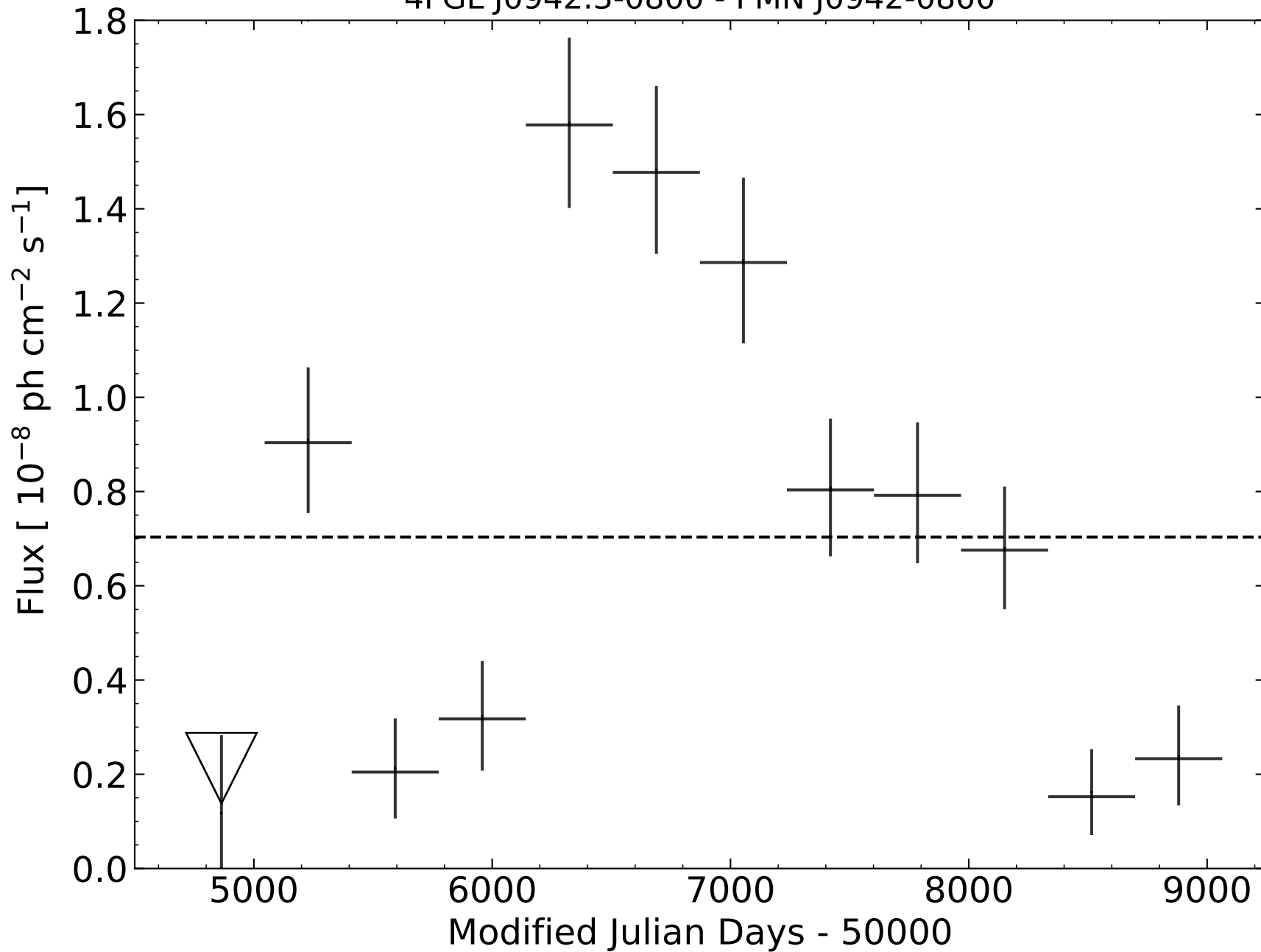
4FGL J0942.3-0800 - PMN J0942-0800
